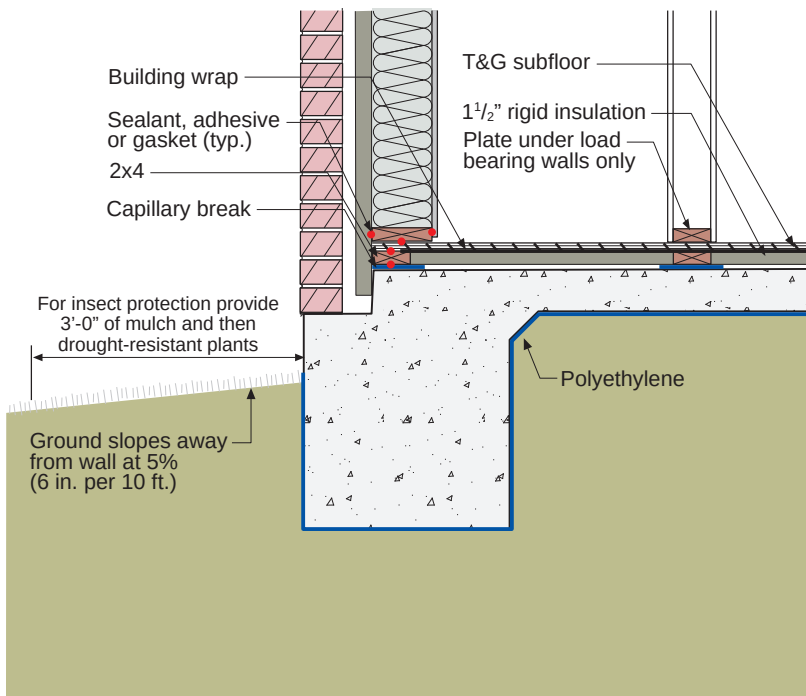
Figure 6.21: Topside Insulated Monolithic Slab Foundation – Mineral Wool Rigid Insulation
