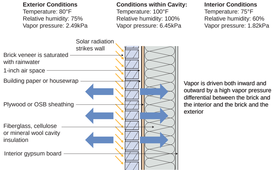
Figure 3.63: Reservoir Claddings - Brick veneer becomes saturated after a rainstorm. The brick acts as a reservoir storing water. When the sun shines on the rain wetter brick veneer it raises the temperature of the water stored in the brick. This water is now driven out of the brick in both directions.
