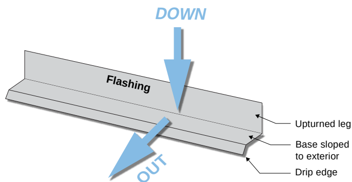
Figure 3.11: Flashings – Direct water downward and outward.
