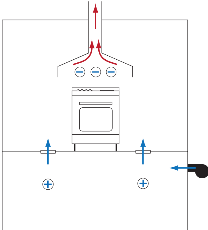
Figure 7.16: Make-Up Air for Vented Kitchen Range Hoods – Approach with basement foundations.
