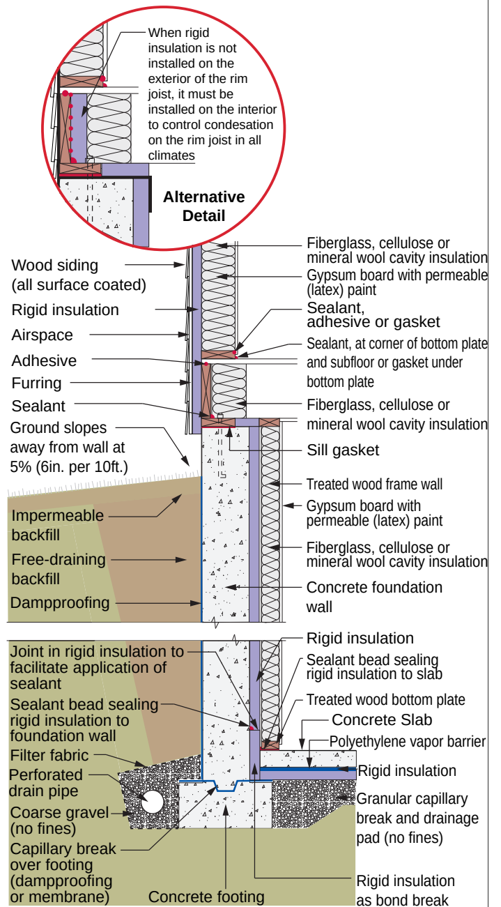
Figure 10.5: Basement Foundation – Internally insulated.
