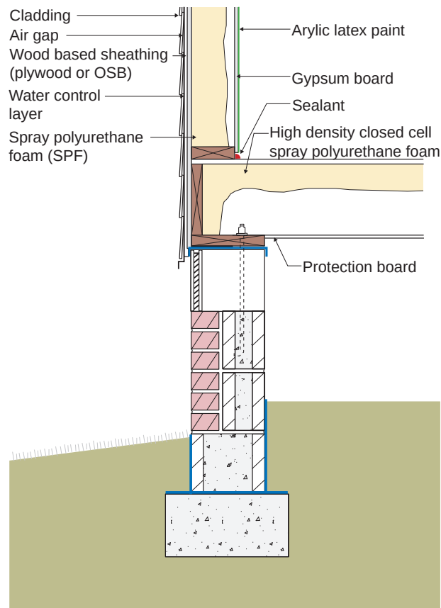
Figure 6.10: Vented Crawlspace – Spray Polyurethane Foam
