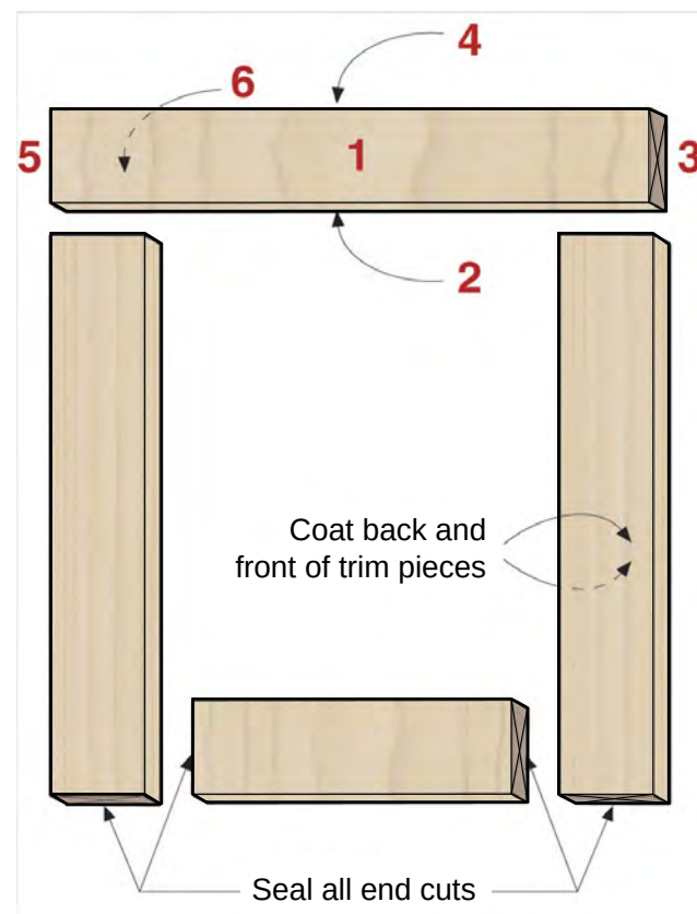
Figure 11.29: Trim Details - Seal or coat all six surfaces of materials to limit water absorption. Back ventilate trim materials so that absorbed water can evaporate and be vented to the exterior.
