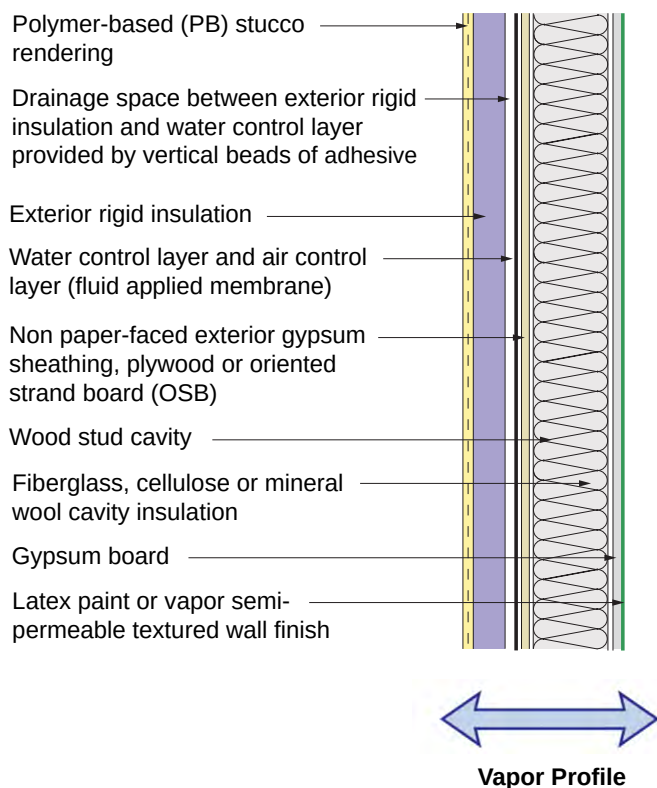
Figure 4.17: Wood Frame Assembly With Exterior Insulation and Interior Cavity Insulation With Stucco
