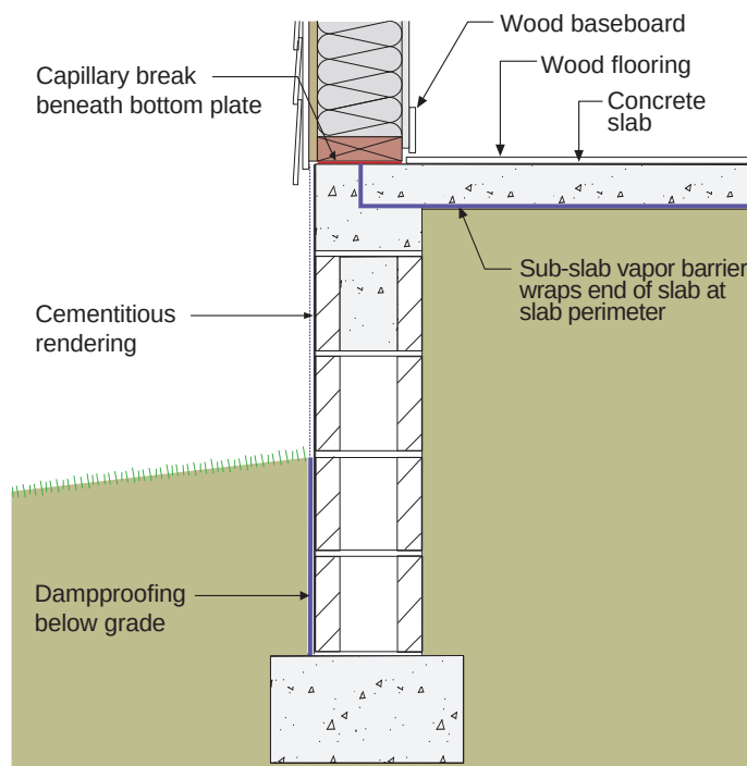
Figure 11.19: Stem Wall Foundation: It is a lot easier to handle a stem wall foundation where the edge of the slab is wrapped and the slab is well elevated.
