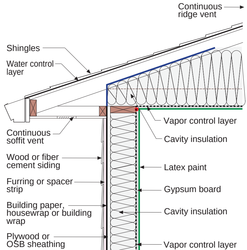
Figure 10.9: Vented Attic – Balanced attic ventilation.
