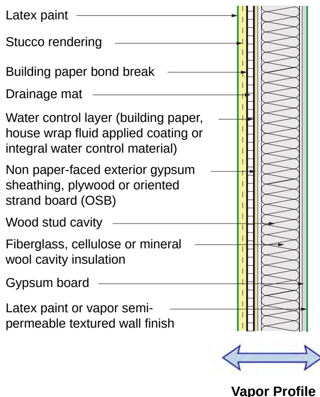
Figure 4.8: Wood Frame Assembly With Interior Cavity Insulation and Stucco
