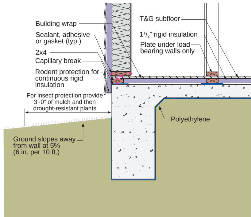
Figure 6.20: Topside Insulated Monolithic Slab Foundation - XPS or EPS Rigid Insulation
