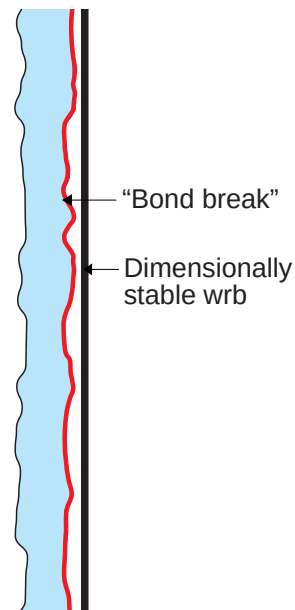
Figure 11.26: Bond Break - It became clear that there were issues with building papers and the first intervention was to use two layers – an outer layer that would act as a bond break and an inner layer that was the “true” water control layer.
