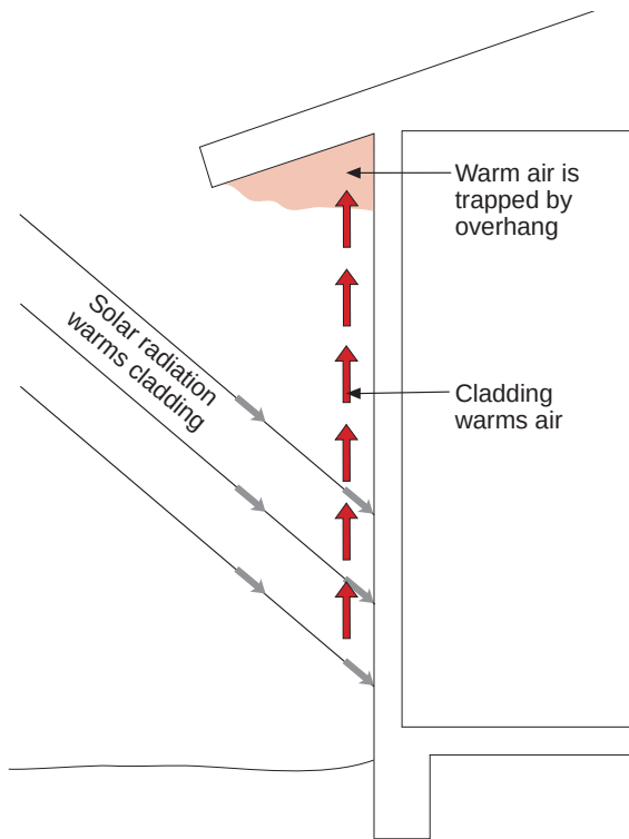
Figure 11.14: Cladding Thermal Plumes – Dark cladding, solar radiation and large over-hangs combine to create ice-dam heaven.
