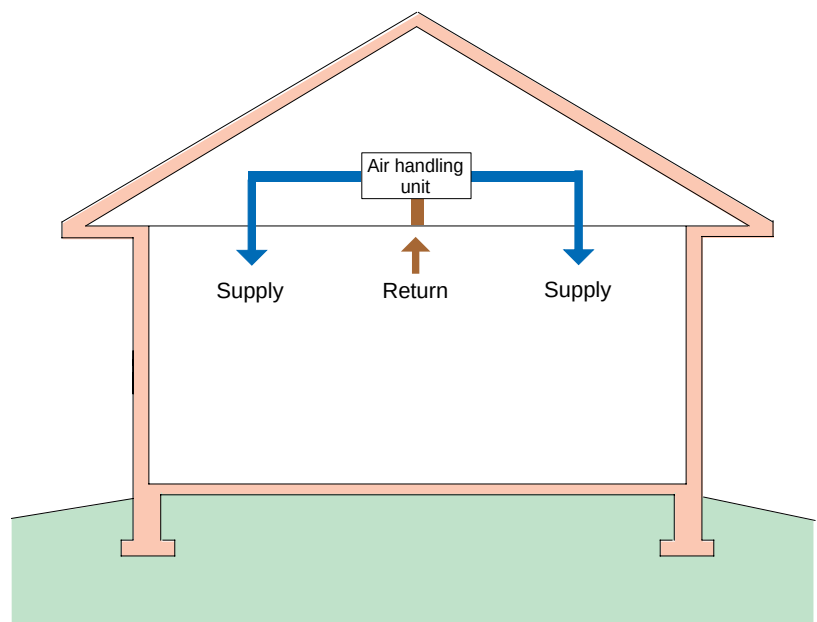
Figure 11.12: Conditioned Attic – Putting the ducts inside by moving the thermal boundary and pressure boundary to the roof deck. This can be done by insulating on the top of the deck or applying spray foam on the underside of the deck.
