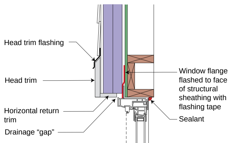
Figure 11.5: Window Head - The window head – the flange at the top of the window – is flashed to the face of the structural sheathing/water control layer and air control layer behind the continuous insulation. A gap is left at the inboard side of the horizontal return trim at the top of the window opening to let any penetrating rainwater run out between the window flange and the horizontal trim.
