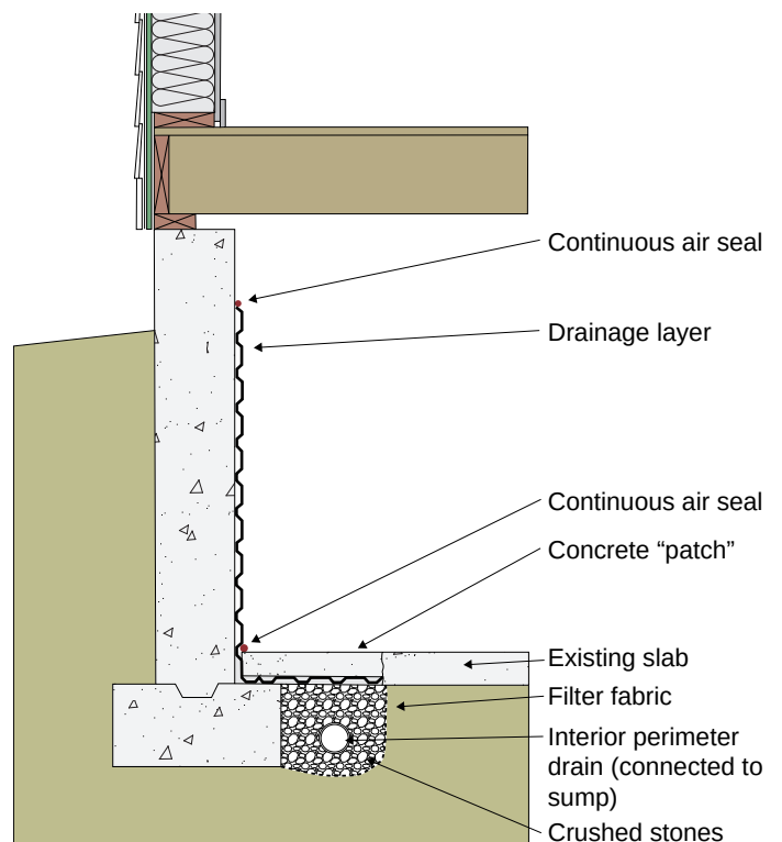
Figure 3.30: Interior Drainage – May be only option for remediation and rehabilitation work.
