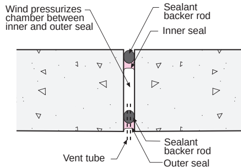
Figure 3.20: Two-Stage Joint – Continuous inner seal and a drained and vented cavity between the continuous inner seal and a weeped outer seal.
