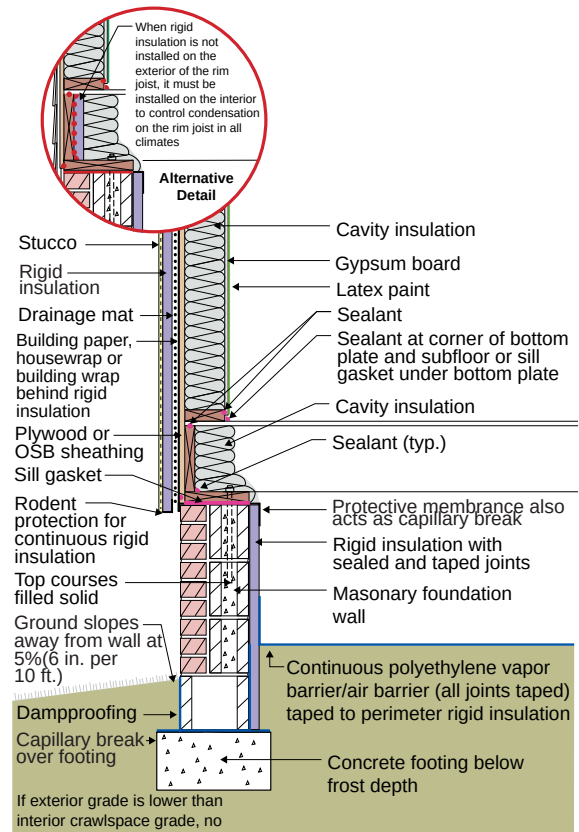
Figure 8.7: Crawl Space Foundation – Conditioned crawl space
