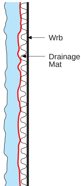
Figure 11.27: Drainage and Drying Gap - The assemblies needed enhanced drainage and enhanced drying. One of the more effective means of accomplishing both is to provide a drainage matt between the bond break and the water control layer.
