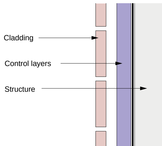
Figure 4.1: Control Layers – Optimum configuration is to place the control layers on the outside of the structure.
