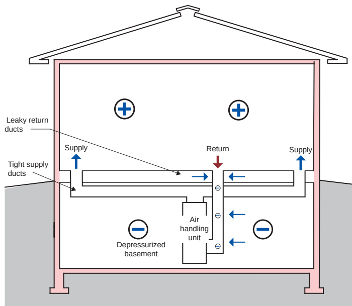
Figure 3.53: Basement Depressurization – Leaky ductwork and unbalanced air flows.
