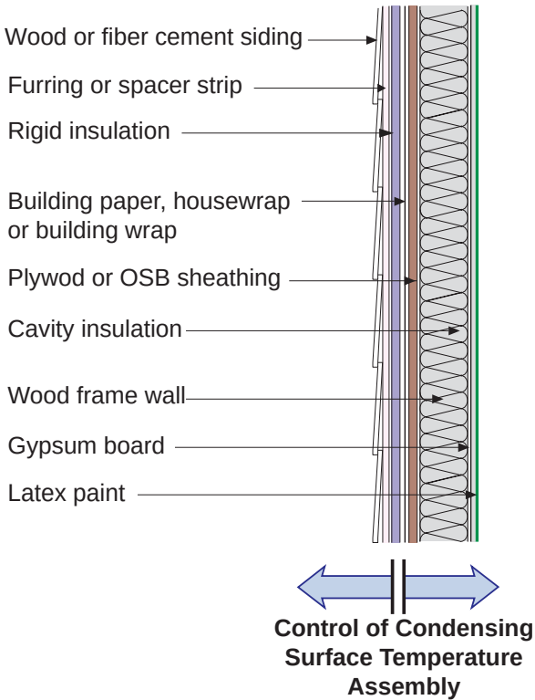
Figure 9.10: Wood Frame Wall – Control of condensing surface temperature assembly.
