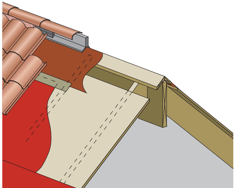
Figure 5.13: Vapor Diffusion Vent – Approach using tile roofing.
