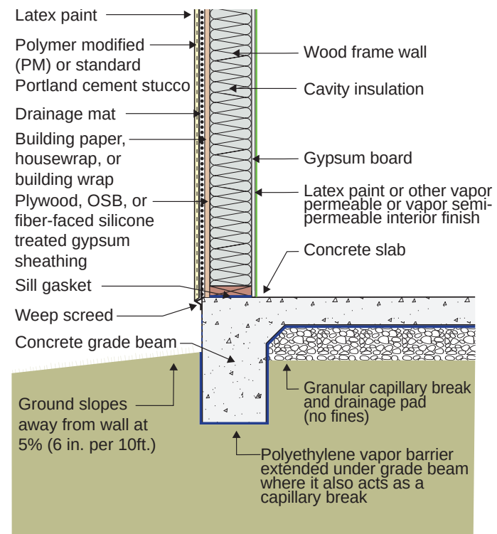
Figure 8.3: Slab Foundation - Frame wall assembly.
