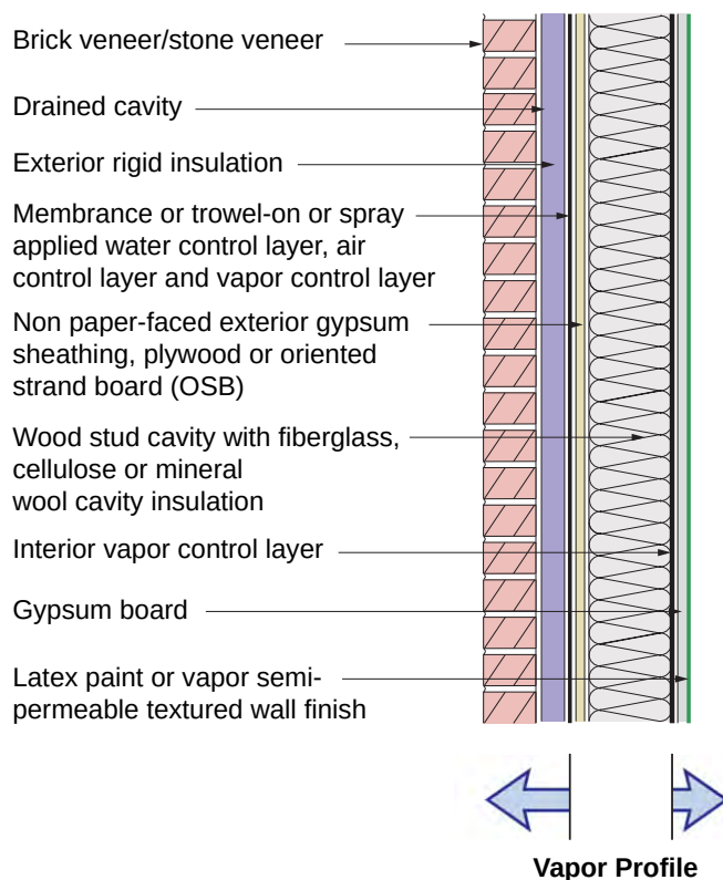
Figure 4.12: Wood Frame Assembly With Exterior Insulation and Interior Cavity Insulation With Brick or Stone Veneer and an Interior Vapor Control Layer
