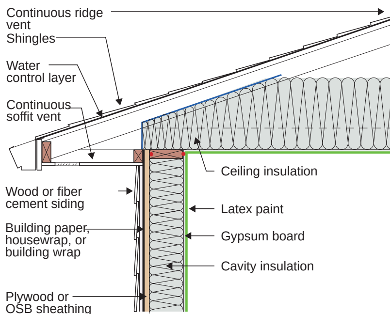
Figure 8.11: Vented Attic – Asphalt shingles.
