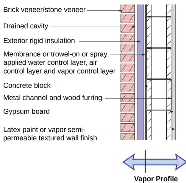
Figure 4.18: Concrete Masonry Unit (CMU) With Exterior Insulation and Brick or Stone Veneer
