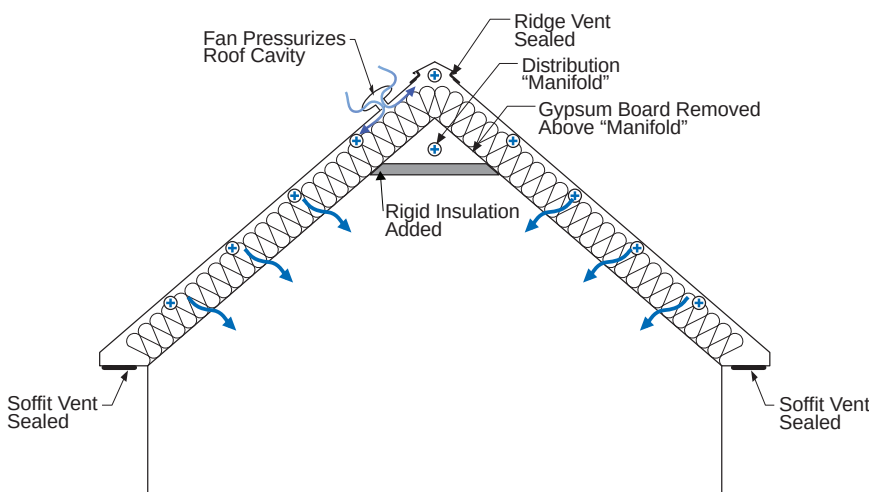
Figure 3.60: Pressurization of Building Assemblies - In cold climates exterior air can be used to pressurize assemblies such as roofs to prevent the migration of air transported moisture from the conditioned space into the assembly.
