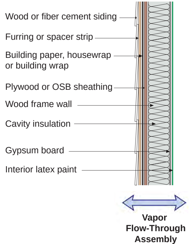
Figure 9.7: Wood Frame Wall – Vapor flow-through assembly.
