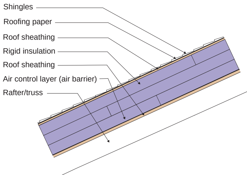
Figure 5.2: Unvented Roof – Sloping roof with all insulation located above the roof deck.
