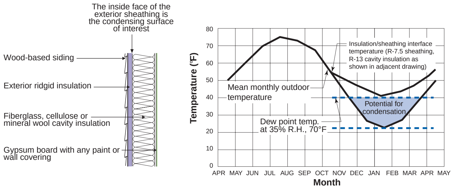
Figure 3.70: Rigid Insulation Reducing Potential for Condensation - Rigid insulation installed on the exterior of the structural framing raises the temperature of the condensing surface of interest controlling condensation from interior water vapor migrating into the wall assembly. This allows assemblies to be constructed in cold climates without interior vapor control layers.
