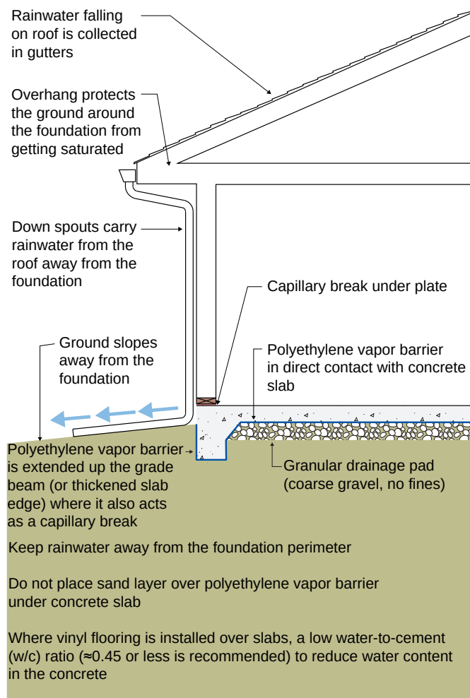
Figure 3.26: Slab-on-Grade – Water management for slab-on-grade construction.
