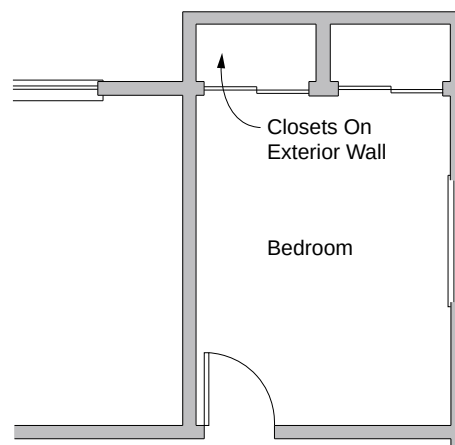
Figure 2.16: Partial Plan of House - Exposed closet on an exterior wall.
