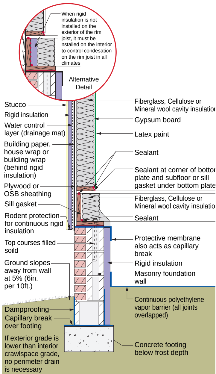
Figure 10.4: Crawl Space Foundation – Conditioned crawl space.
