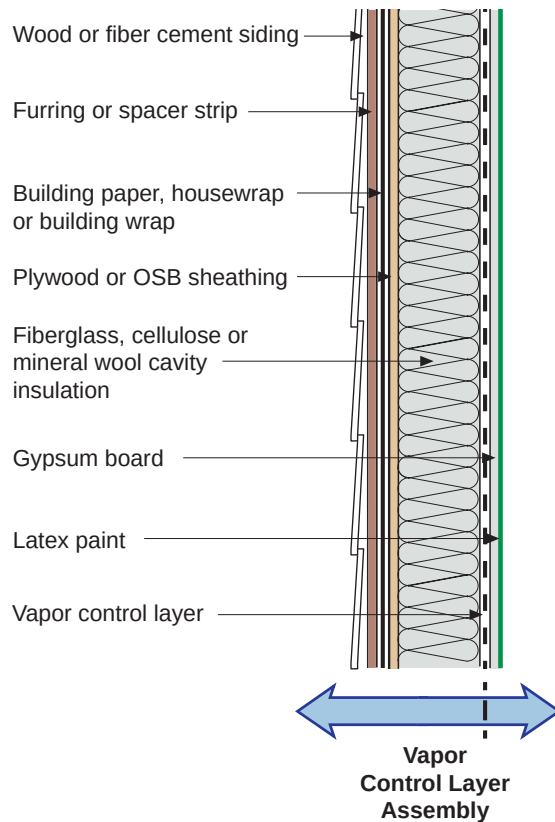
Figure 3.64: Interior Vapor Control Layer Assembly – Wall with vapor control layer on the interior of wall cavity insulation.
