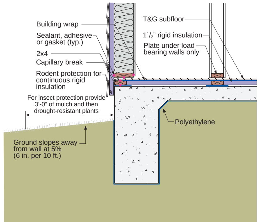
Figure 6.22: Topside Insulated Monolithic Slab Foundation with Brick Veneer - XPS or EPS Rigid Insulation
