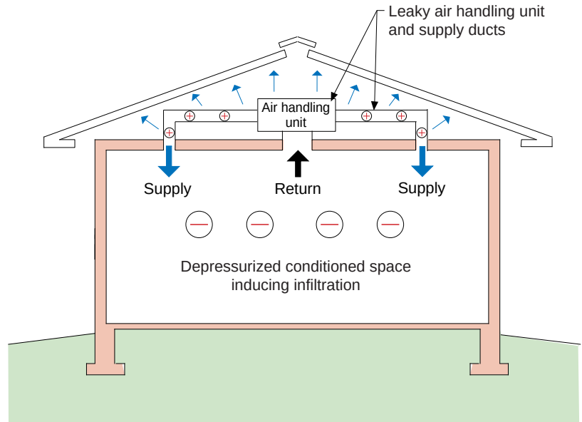
Figure 11.11: Ductwork in Attics - The air leakage out of the ducts and the conductive and radiative losses from the surfaces of the ducts results in ice damming.
