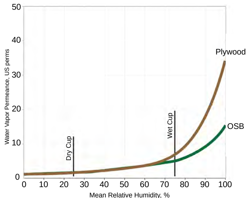
Figure 2.12: Vapor Transmission of Plywood and Oriented Strand Board (OSB) - What makes them work is the wet cup performance not the dry cup performance. Lots of walls would be rotting if they stayed at their dry cup value regardless of the relative humidity and their respective moisture contents.
