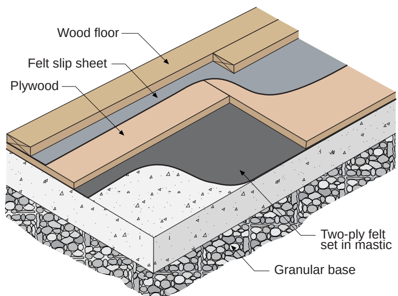
Figure 11.15: Historic Practice: A continuous layer of bitumen was installed over the top of the concrete surface. The bitumen would be both a vapor barrier and a capillary break. To keep it from getting over everything it was covered with felt paper. Sometimes installed in two layers.
