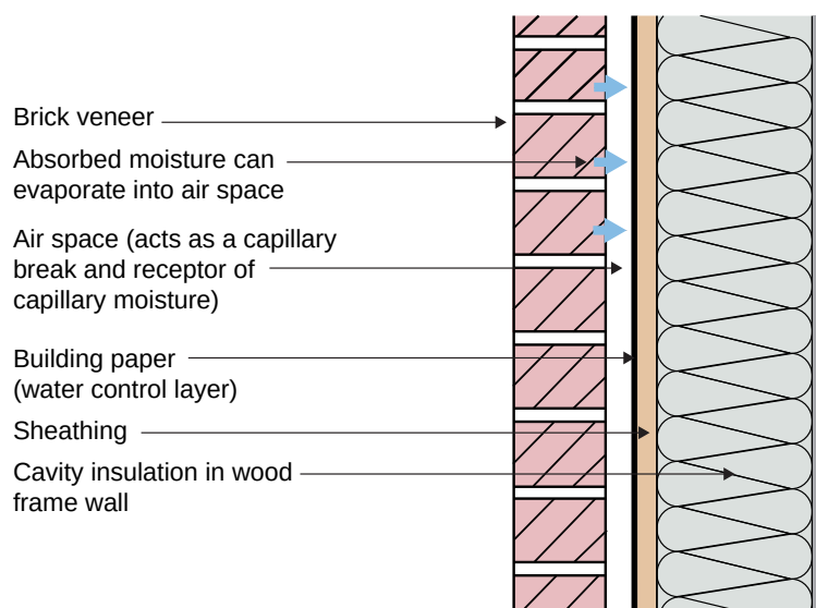
Figure 3.36: Brick Veneer - Air space serving as a capillary break as well as serving as a receptor for capillary moisture.
