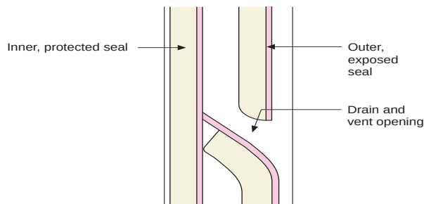
Figure 3.21: Two-Stage Joint Section - Section through a two-stage joint that uses sealant to direct water to the exterior.
