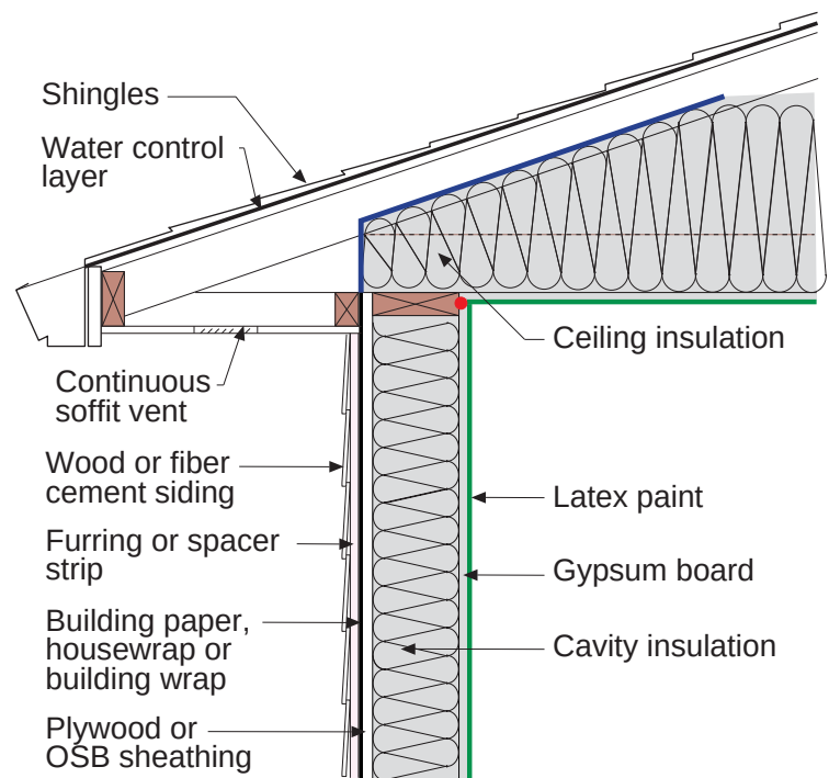
Figure 9.11: Vented Attic – Balanced attic ventilation.
