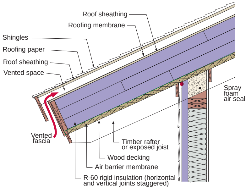
Figure 11.13: Compact Roof – Roof deck insulated on the topside. Note the air control layer. Note that the air intake for the vented “over-roof” is at the fascia and that the over-hang is insulated compensating for cladding thermal plumes due to incident solar radiation.
