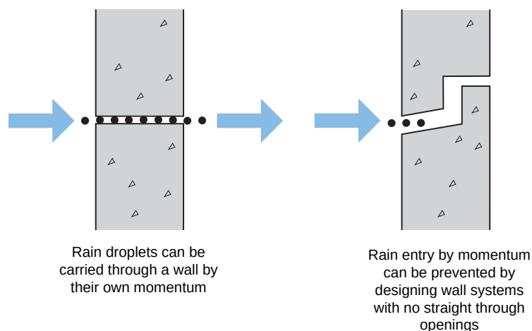
Figure 3.3: Momentum - A driving force for rain entry.
