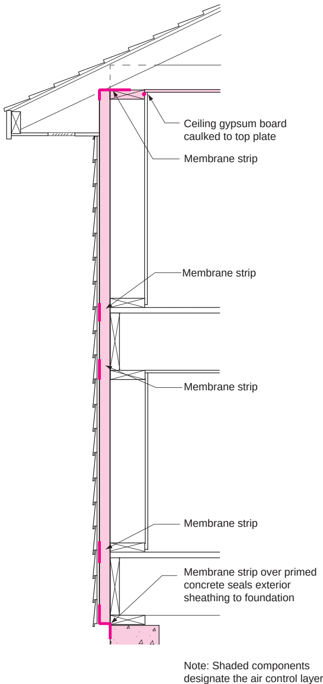
Figure 3.47: Exterior Air Control Layer - Exterior continuous rigid insulation can also be sealed to the framing elements to act as an exterior air control layer.
