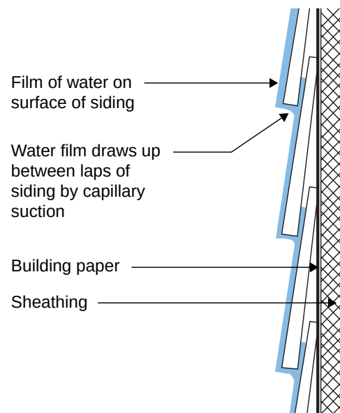
Figure 3.33: Capillarity Above Grade - Water trapped between the laps in horizontal wood siding.
