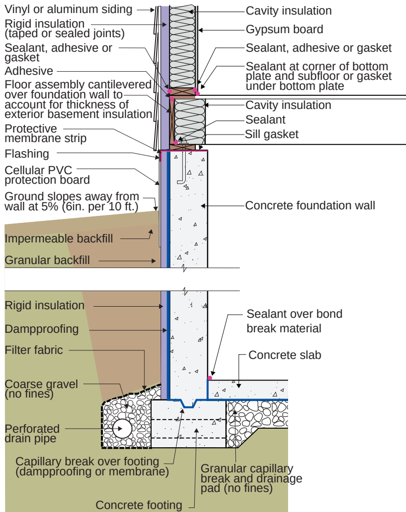
Figure 6.7: Concrete Basement With Exterior Rigid Insulation
