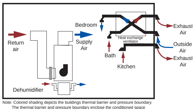
Figure 7.15: Balanced Ventilation - Approach using an energy recovery ventilator (ERV), a vented range hood and supplemental dehumidification.
