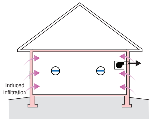
Figure 7.7: Dilution Ventilation – Exhaust system approach.
