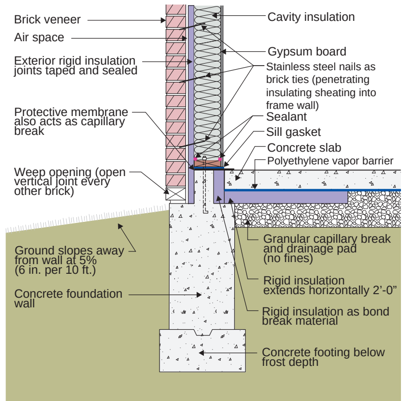
Figure 8.5: Stem Wall Foundation – Internally insulated stem wall foundation with brick veneer.
