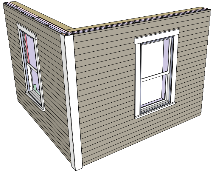
Figure 11.31e: Cladding Installed – Sealed on all six sides over an air gap.
