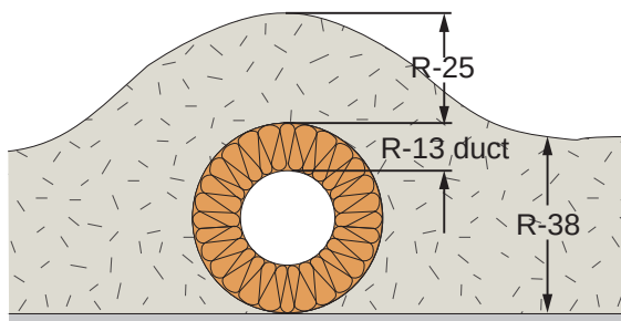
Figure 5.14: Buried Ducts – Approach for hot-humid and mixed-humid climates
