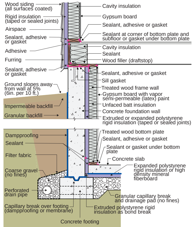
Figure 6.6: Concrete Basement With Interior Rigid Insulation and an Interior Insulated Frame Wall
