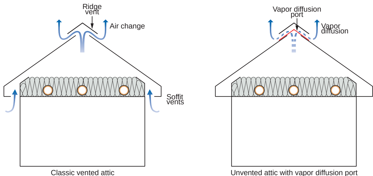
Figure 5.16: Buried Ducts – Alternative approach for hot-humid and mixed-humid climates.
