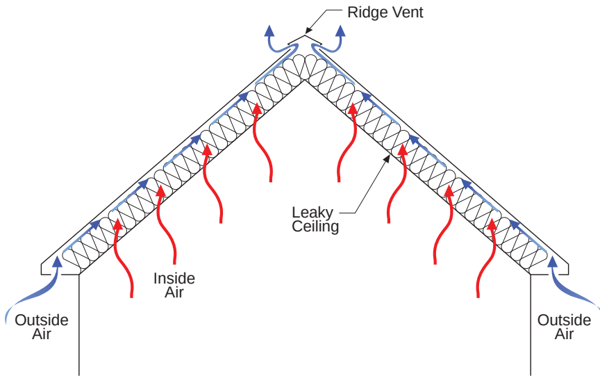
Figure 3.59: Air Leakage of Cathedral Ceiling – Cold climate condensation issue.
