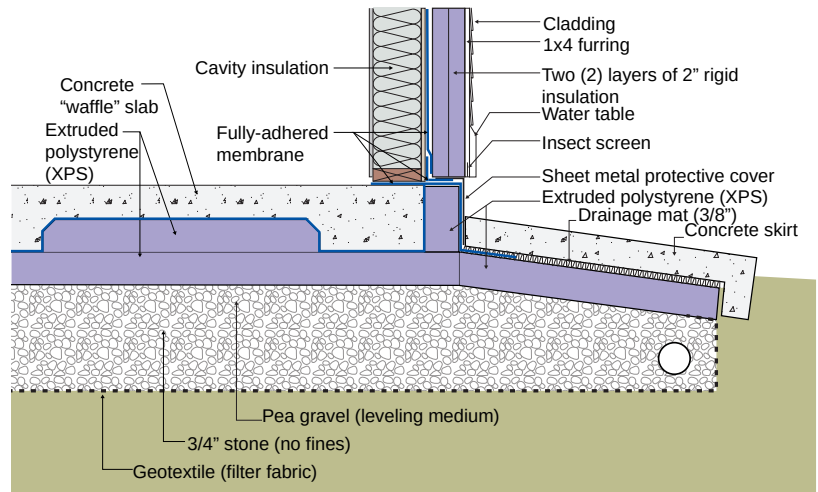
Figure 6.24: Shallow Frost Protected Slab Foundation – XPS or EPS Rigid Insulation
