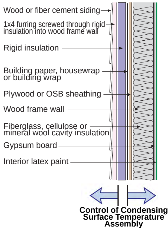
Figure 10.7: Wood Frame Wall – Control of condensing surface temperature assembly.
