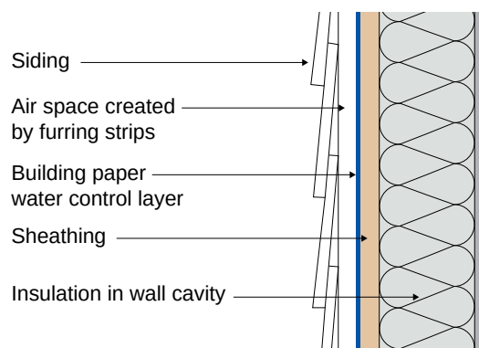
Figure 3.35: Capillary Control Above Grade - The paint film seals the capillary pores on the surface of the wood. Additionally, the siding should be installed over an air space behind the siding to act as a receptor for capillary moisture.
