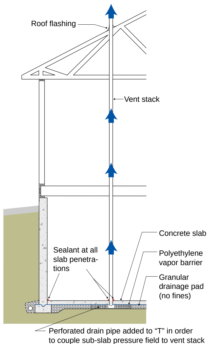
Figure 6:3: Soil Gas Control – Approach for basement foundations.
