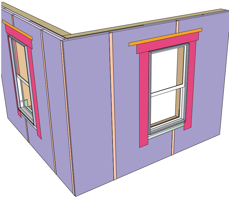
Figure 11.31a: Continuous Exterior Insulation – Water control layer is the exterior face of the insulation. Note the taped joints.
