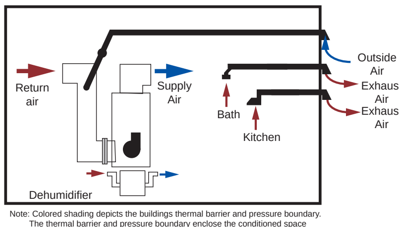
Figure 7.14: Balanced Ventilation – Approach using outside air to the return side of the air handler coupled with bathroom fans, a vented range hood and supplemental dehumidification.
