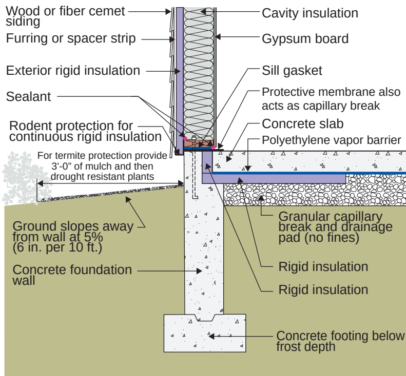
Figure 8.4: Stem Wall Foundation – Internally insulated.
