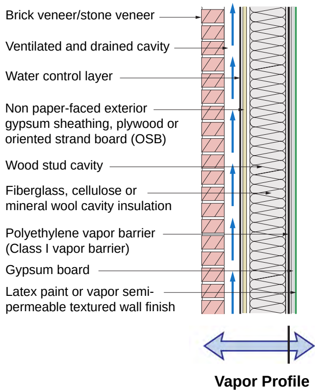
Figure 4.5: Wood Frame Assembly With Interior Cavity Insulation and Brick or Stone Veneer With an Interior Vapor Control Layer.
