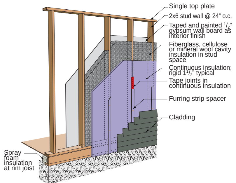
Figure 11.2: Continuous Insulation as the Water Control Layer and Air Control Layer - Include or exclude the structural sheathing based on structural considerations.
