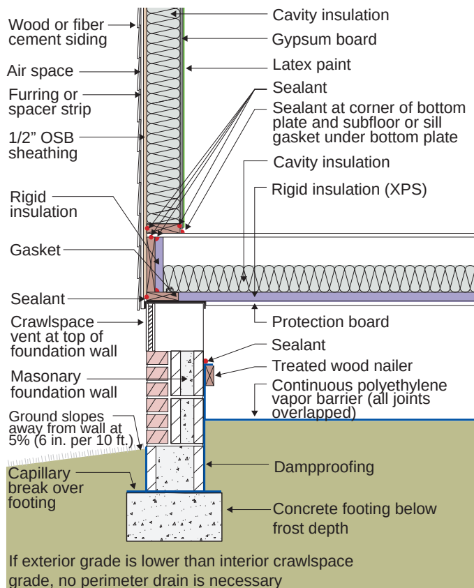
Figure 8.6: Crawl Space Foundation – Vented crawl space.
