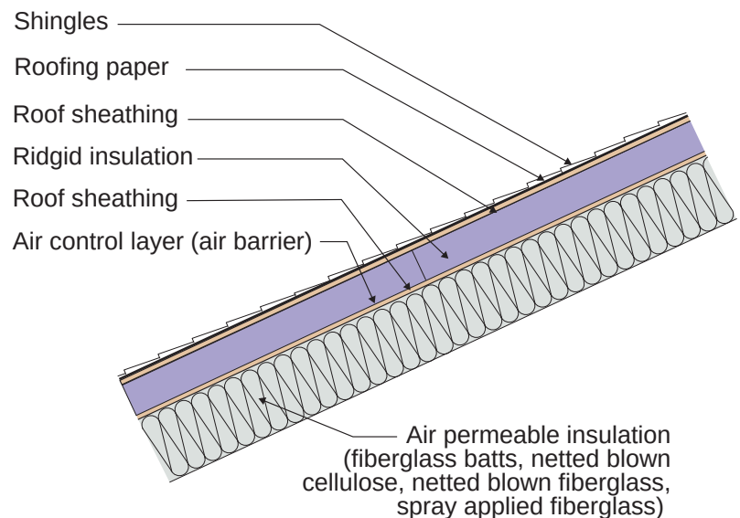
Figure 5.8: Unvented Attic – Roof with some insulation can be located above the top of the roof sheathing and some of the insulation can be located on the underside of the roof sheathing.
