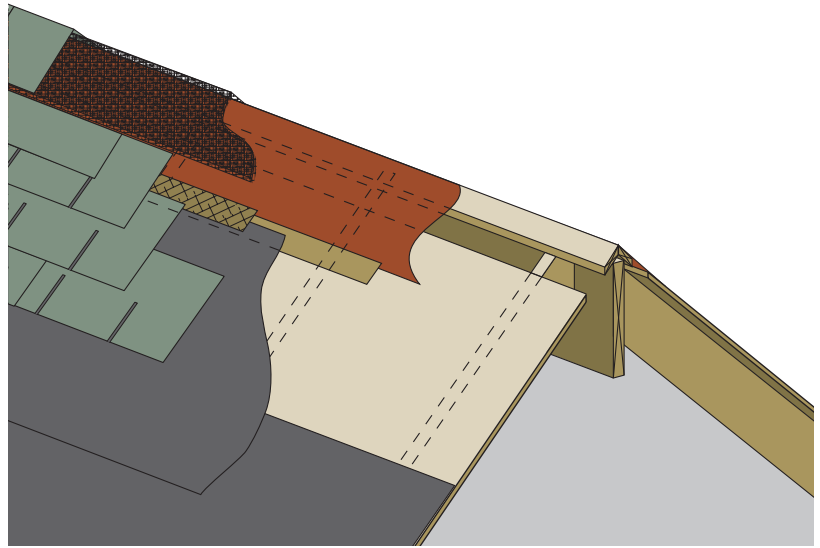
Figure 5.12: Vapor Diffusion Vents – Approach using asphalt shingles.
