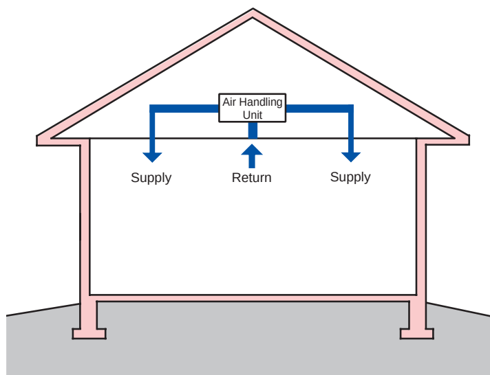
Figure 3.55: Depressurization of Slab Buildings – Leaky ductwork located in vented attics leads to depressurization.
