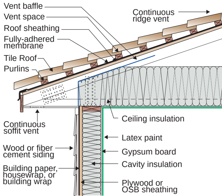
Figure 8.12: Vented Attic – Tile roof covering.
