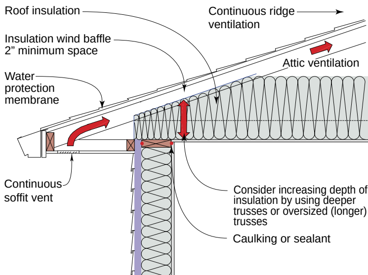
Figure 11.10: Classic Control Approach - Keep heat from the interior from getting to the roof deck and then remove any heat that gets there. First, construct an airtight “lid” or ceiling plane. Second, insulate the top of the lid with insulation. And then third, flush away any heat that gets to the roof deck by ventilating the underside of the roof deck with exterior air. Note the air seals at the top of the exterior wall. Exterior walls are like chimneys – you don’t want to vent the tops of them into your roof. The minimum thermal resistance directly over the top of the top plate should be greater than the thermal resistance of the wall. Also, note that a 2 inch minimum airspace is recommended under the sheathing
