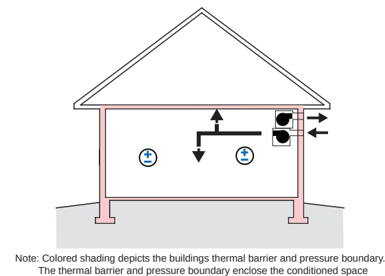
Figure 7.8: Dilution Ventilation – Supply system approach.
