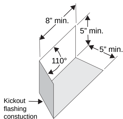
Figure 3.15: Kickout Flashing: The name describes the function. Rainwater running down the slope of the roof is directed away from the wall at the bottom of the roof – it is “kicked out” of the wall at the roof wall intersection.
