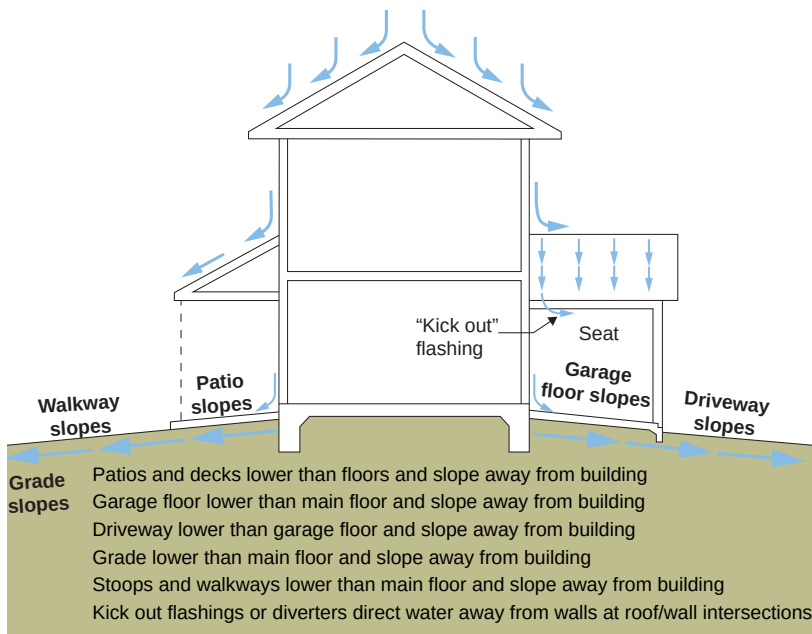
Figure 3.13: Drain the Building – Layer the levels and drain away from the building.
