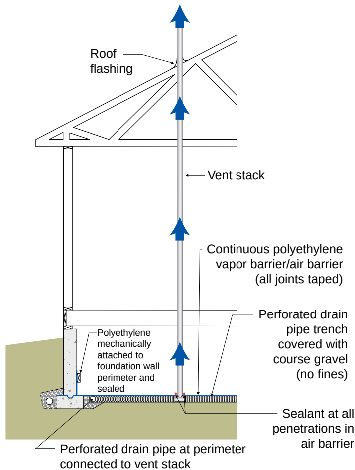
Figure 6.2: Soil Gas Control – Approach for crawl space foundations.
