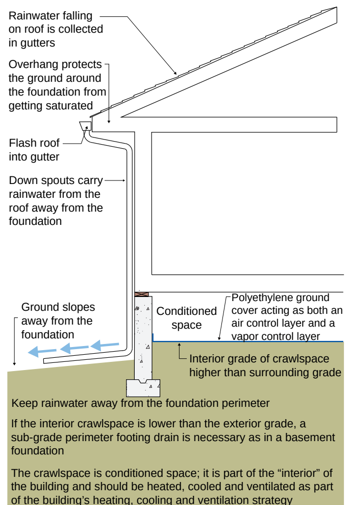
Figure 3.27: Crawl Space – Water management for crawl space construction.
