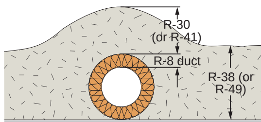
Figure 5.15: Buried Ducts – Approach for colder climates.
