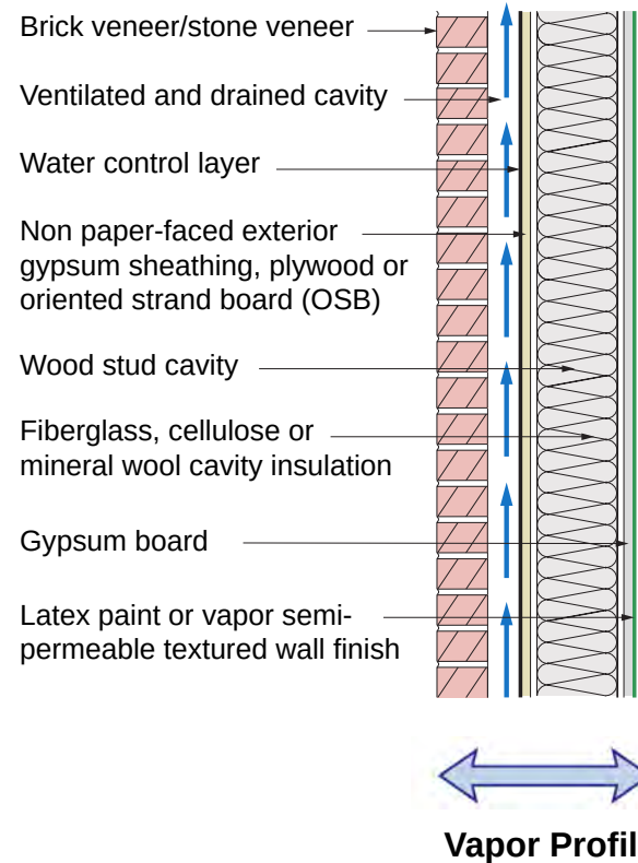
Figure 4.3: Wood Frame Assembly With Interior Cavity Insulation and Brick or Stone Veneer
