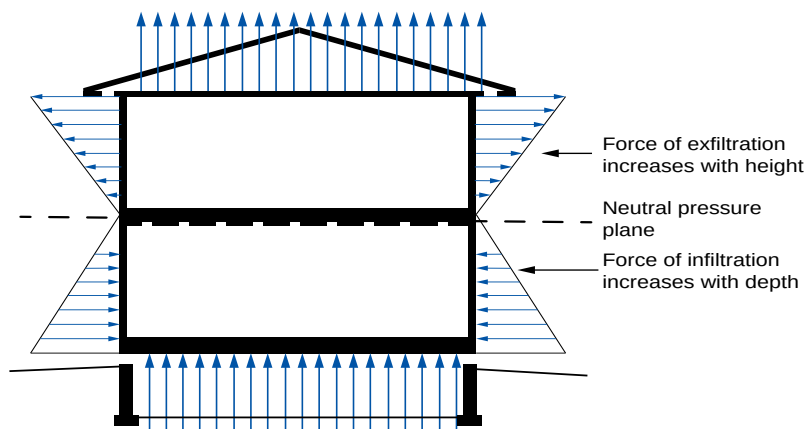
Figure 3.48: Stack Effect - The upper portion of the building, inside air pressure is greater than outside air pressure, leading to exfiltration. At the lower portion of the building, inside air pressure is lower than outside air pressure, leading to infiltration.
