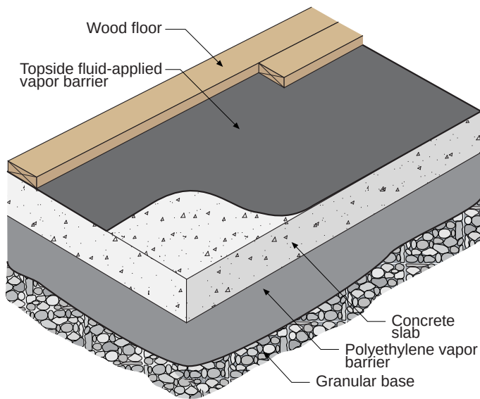
Figure 11.21: What if Your Slab is Wet?: A topside vapor barrier should be installed. A fluid applied vapor barrier such as epoxy work well.
