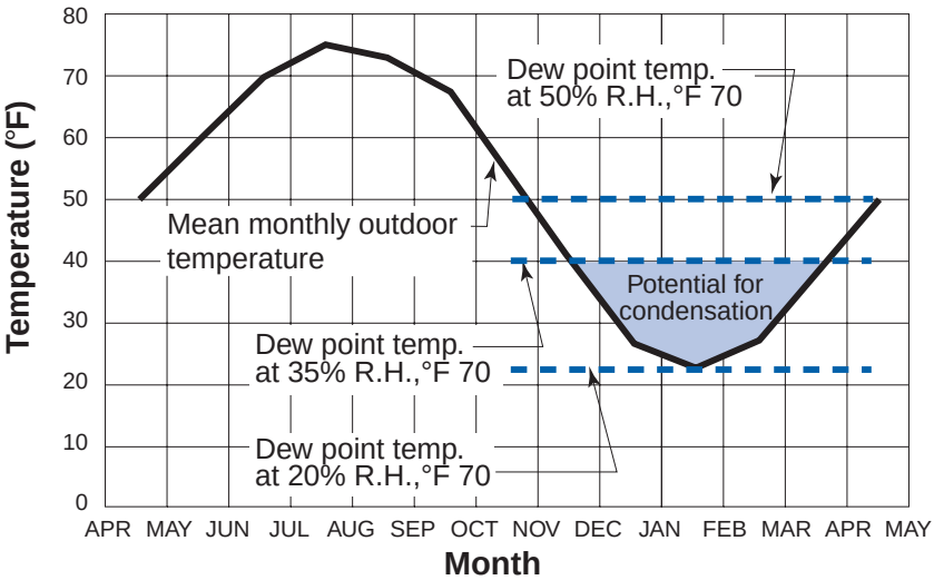
Figure 3.69: Potential for Condensation - Potential for condensation for a wall assembly located in Chicago, IL with various levels of interior RH.
