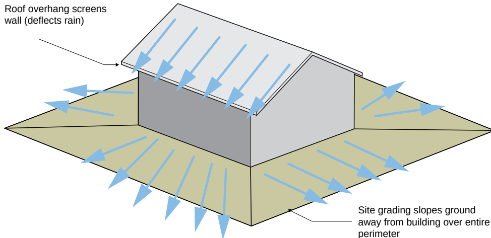
Figure 3.25: Site Grading - Site grading is used to direct surface water away from building foundations.
