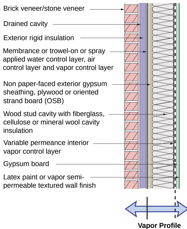
Figure 4.13: Wood Frame Assembly With Exterior Insulation and Interior Cavity Insulation With Brick or Stone Veneer and a Variable Permeance Interior Vapor Control Layer or Kraft Faced Cavity Insulation
