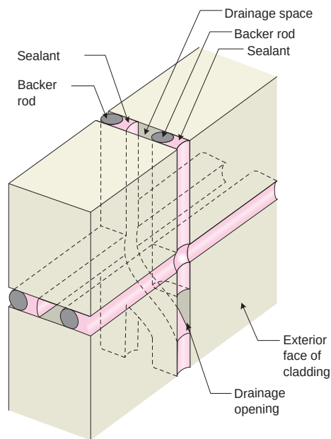
Figure 3.22: Three Dimensional Detail of Two-Stage Joint - Drainage paths are shown. The outer seal is exposed to the elements – ultra violet light, heat and water – but the assembly still works because of the interior protected seal.
