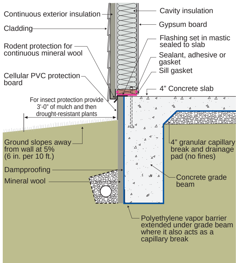
Figure 6.19: Externally Insulated Monolithic Slab Foundation – Mineral Wool Rigid Insulation
