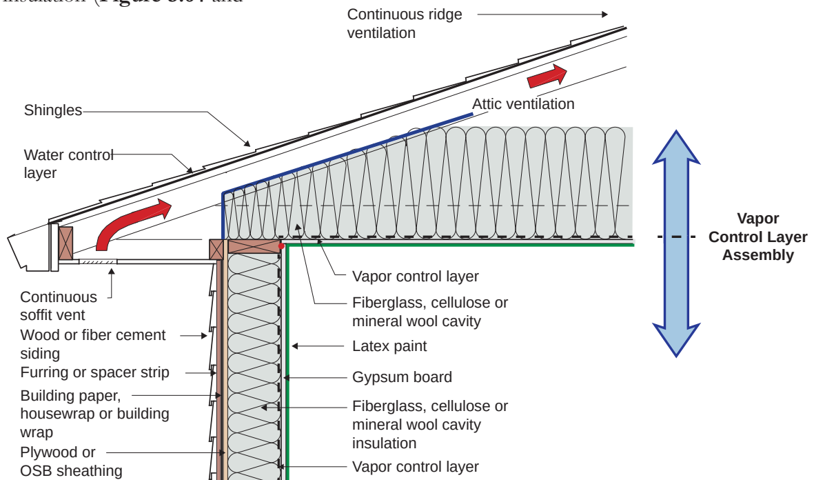
Figure 3.65: Interior Vapor Control Layer Assembly – Attic with vapor control layer at the underside of attic insulation.
