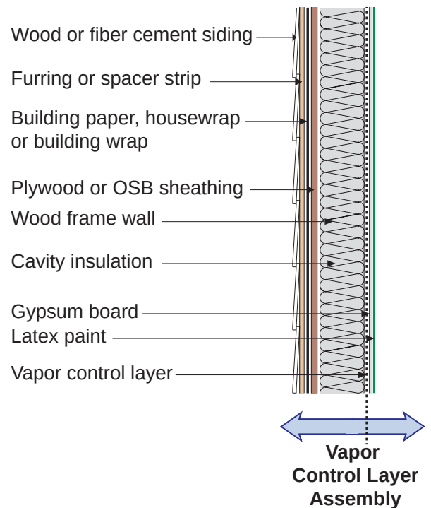
Figure 9.8: Wood Frame Wall – Vapor control layer assembly.
