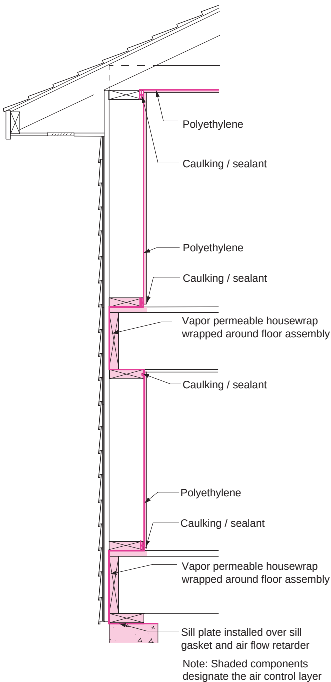
Figure 3.42: Interior Air Control Layer - Resistance to air flow (airtightness) at the interior of building assemblies in cold climates is typically provided by installing a continuous, sealed polyethylene film between the interior cladding or gypsum board and the framing elements.
