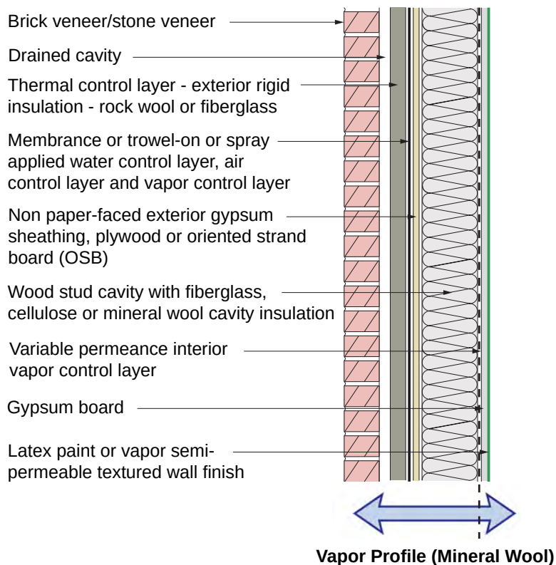
Figure 4.16: Wood Frame Assembly With Exterior Insulation and Interior Cavity Insulation With Brick or Stone Veneer and a Variable Permeance Interior Vapor Control Layer or Kraft Faced Cavity Insulation
