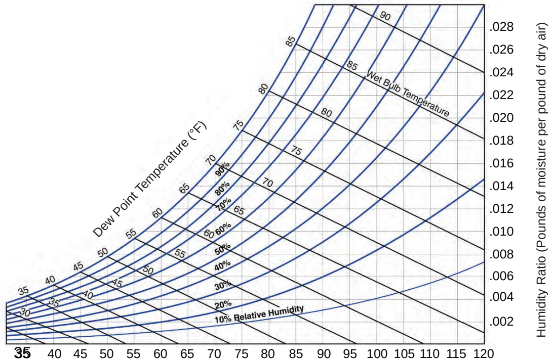
Figure 2.15: Psychrometric Chart - The relationship between temperature, relative humidity and vapor pressure is presented graphically on a psychrometric chart.
