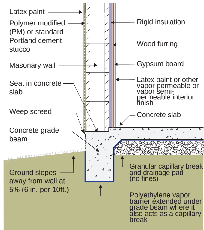
Figure 8.2: Slab Foundation - CMU wall construction.
