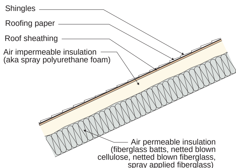
Figure 5.9: Unvented Attic - Spray polyurethane foam on the underside of the roof deck coupled with air permeable insulation. The thermal resistance of the spray polyurethane foam and the thermal resistance of the insulation under it must conform to the ratio stipulated in Table 5.1.
