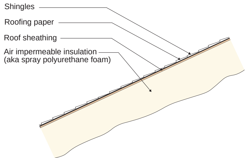
Figure 5.7: Unvented Attic – Roof with all insulation located below the roof deck using spray polyurethane foam insulation.
