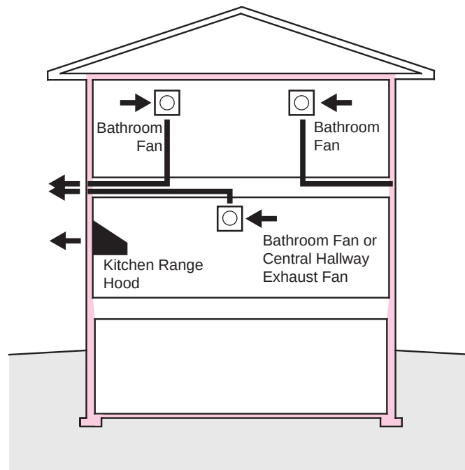
Figure 7.10: Exhaust Only Ventilation – Approach using bathroom fans and vented range hood.
