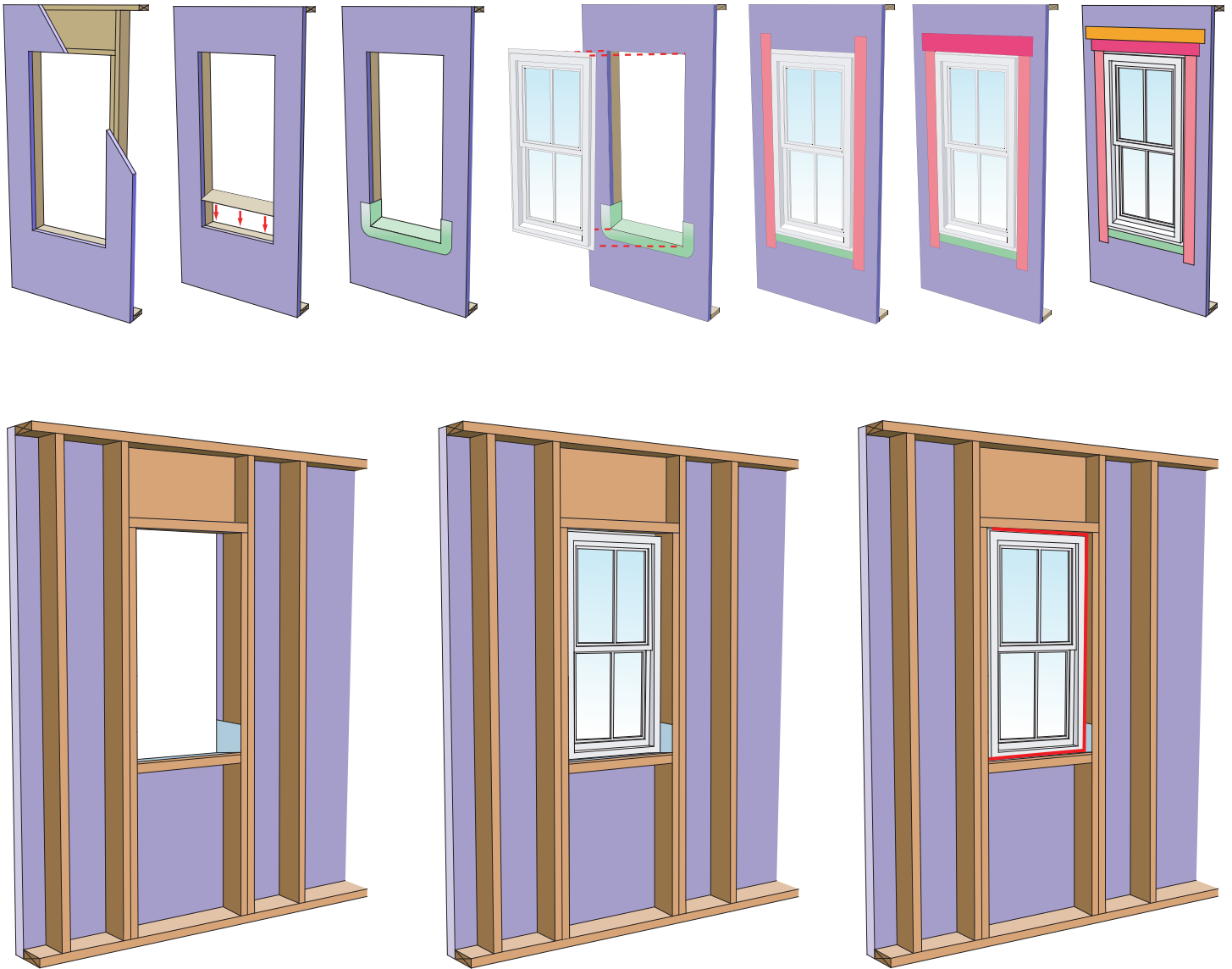
Figure 11.6: Window Installation Sequence For “Outies”. The water and air control layer is the face of the continuous insulation. Note that the water control of the flanged window lines up with the water control of the face of the continuous insulation. Again note that the pan flashing can be liquid applied or a formable membrane. Again note that sealant is not necessary behind the window flanges. And finally note that there is no wood behind the window flange – the flange is seated directly over the continuous insulation. The window is attached through the flange and continuous insulation to the framing with long screws.
