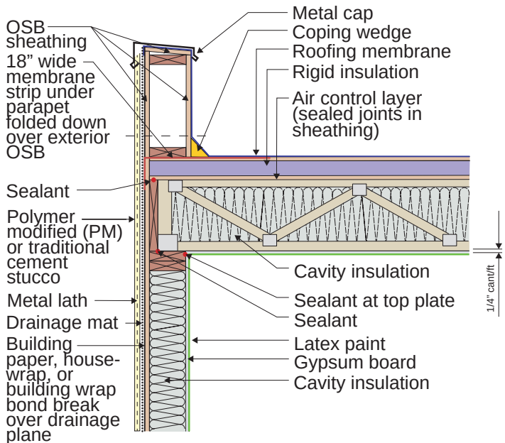
Figure 8.14: Conditioned Attic – Hybrid assembly with insulation located above and below the roof deck.
