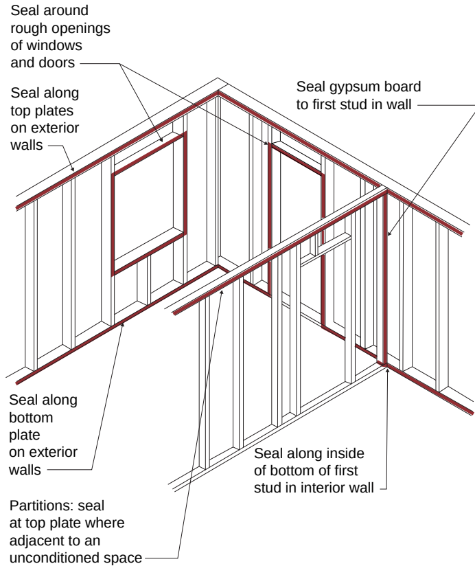
Figure 3.41: Interior Air Control Layer - Interior air control layers need to address air leakage concerns at multiple locations.
