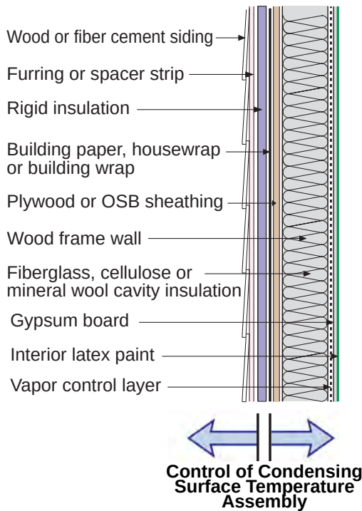
Figure 10.7: Wood Frame Wall – Control of condensing surface temperature assembly.
