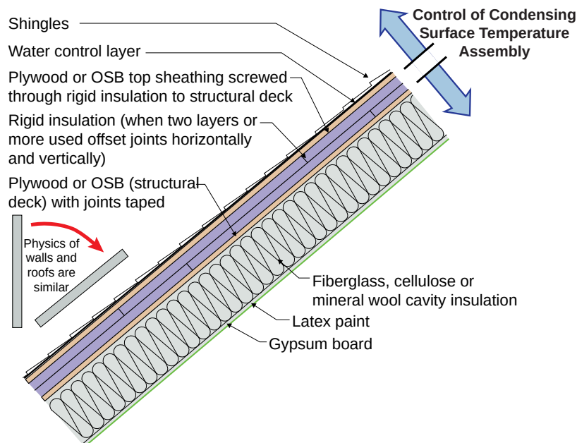
Figure 3.71: Roof Assembly - Rigid insulation is installed over the top of the structural roof deck elevating the temperature of the underside of the roof deck to control condensation.
