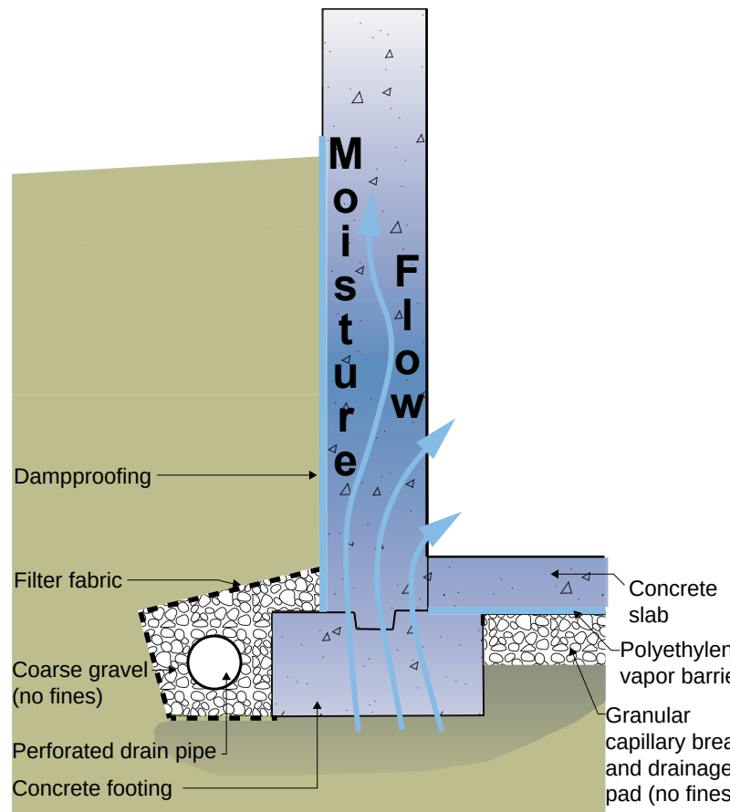
Figure 3.32: Capillarity – Footings typically do not have capillary breaks.
