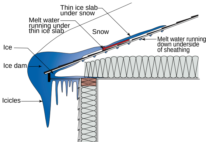
Figure 11.9: Melt Water – When the snow layer adjacent the roof deck melts the liquid water is wicked upward into the snow pack by capillarity away from the roof covering. As the liquid water migrates upwards it gets colder and freezes. As more snow melts and the liquid water phase exceeds the storage capacity of the snow it runs downward under the ice layer via gravity. At the roof edge and roof overhang the deck is much colder and the drainage gap freezes solid causing the water to back up.
