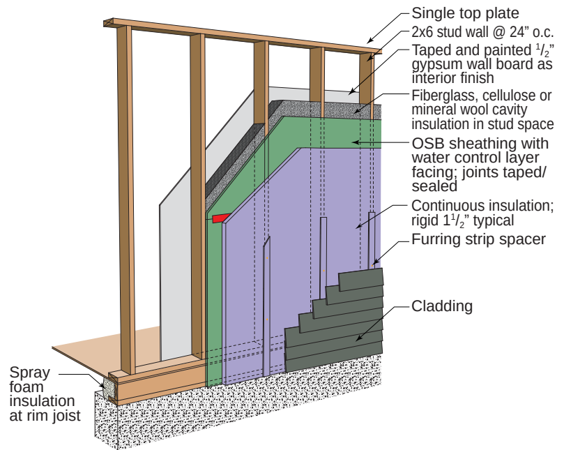
Figure 11.1: Structural Sheathing as the Water Control Layer and Air Control Layer – Continuous insulation is installed over the structural sheathing.
