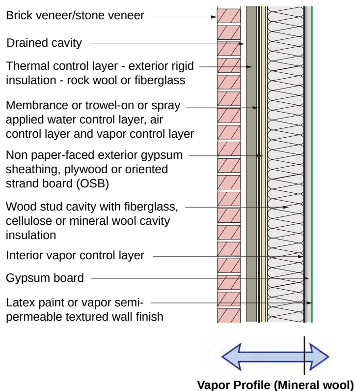
Figure 4.15: Wood Frame Assembly With Exterior Insulation and Interior Cavity Insulation With Brick or Stone Veneer and an Interior Vapor Control Layer
