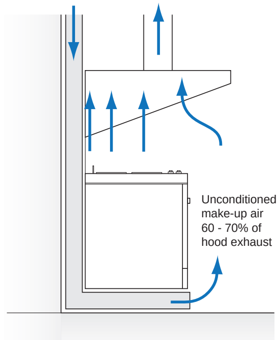
Figure 7.17: Make-Up Air for Vented Kitchen Range Hoods – Approach with slab foundations.
