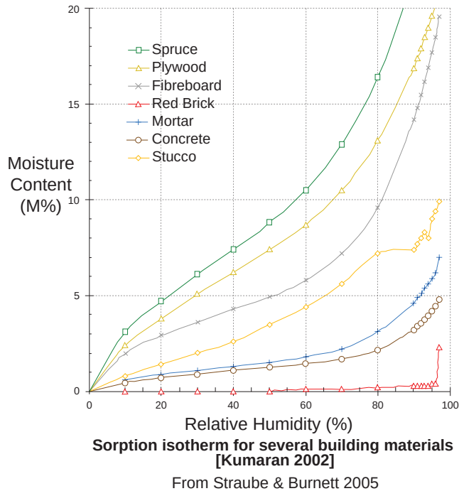
Figure 2.8: Sorption Isotherms - Common building materials sorption isotherms— courtesy of Kumaran by way of Straube and Burnett (2005).
