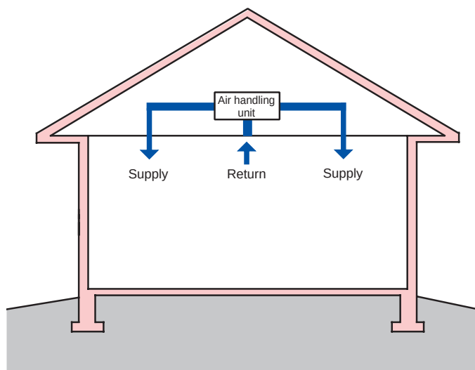
Figure 3.57: Conditioned Attic – Ductwork now located in conditioned space.
