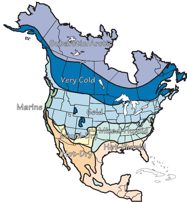
Figure 1.1: Hygrothermal Regions - Based on Herbertson's Thermal Regions and Köppen climate types.
