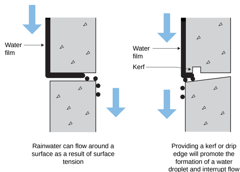
Figure 3.4: Surface Tension – A driving force for rain entry.
