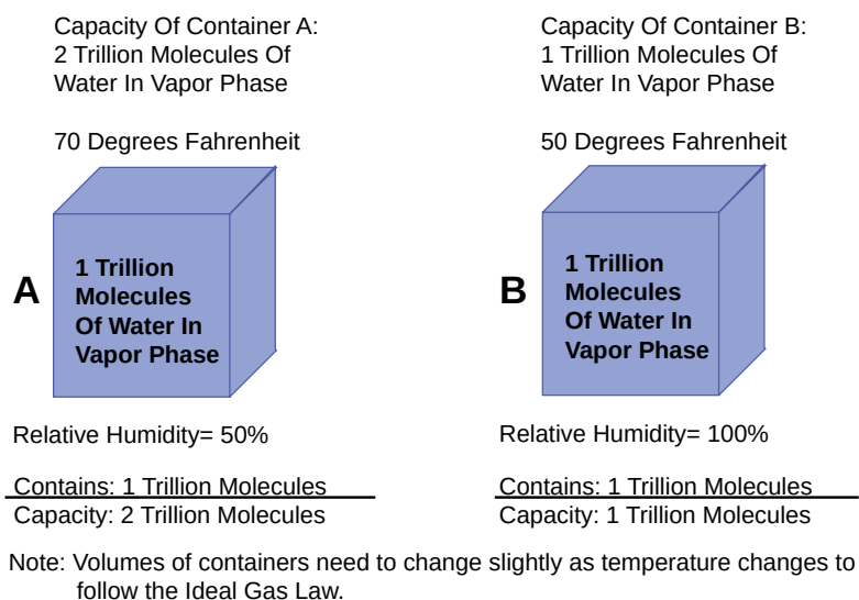
Figure 2.13: Relative Humidity Increases as Temperature Decreases - The concept of relative humidity, vapor pressure, and the influence of temperature and vapor pressure on relative humidity.
