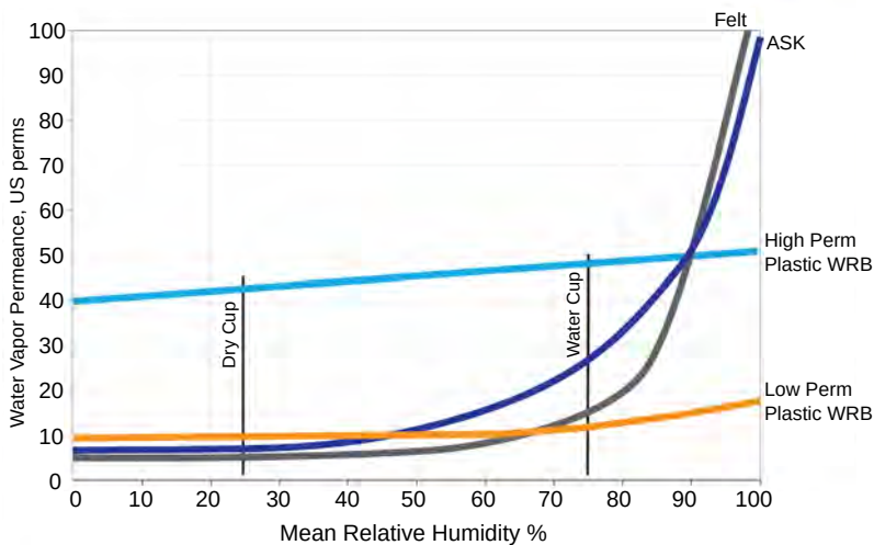
Figure 2.11: Permeance of Exterior Wall Layers - Look at the shape of the curves for the traditional materials: impregnated felt and asphalt saturated kraft (ASK). Notice how the bend upward past 50 percent relative humidity. Hard to knock the old materials. They were pretty darn “smart”.
