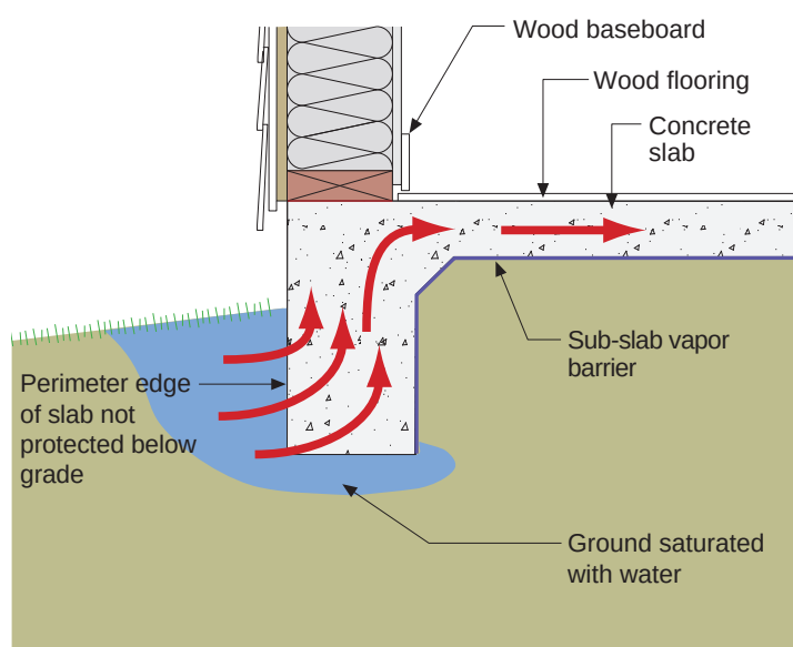
Figure 11.18: Capillary Wicking: Without the slab edge protection water can wick dozens of feet inward via capillarity.
