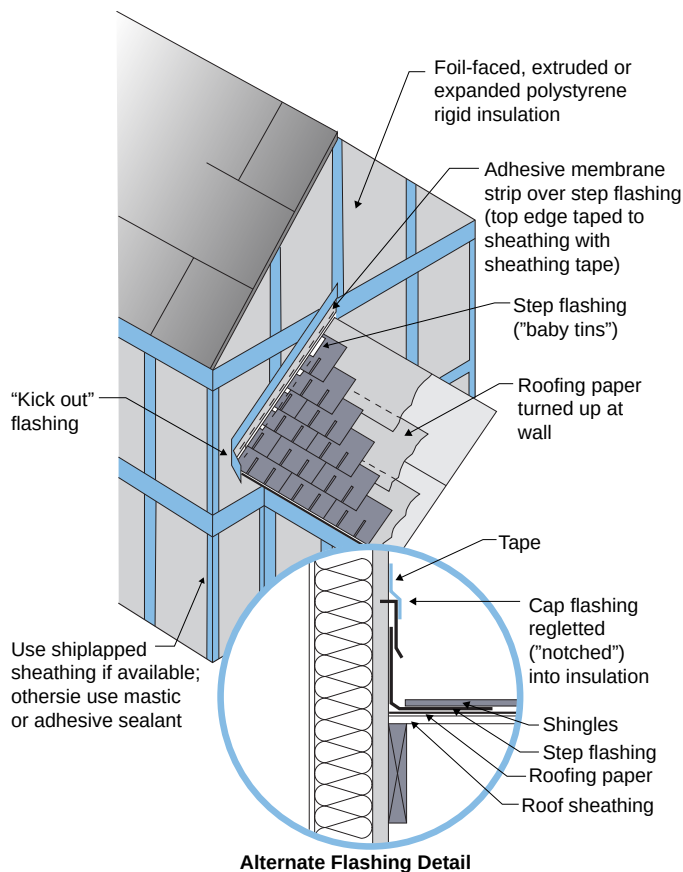
Figure 3.14: Roofs Intersecting Walls: Roofs can also concentrate rainwater where roofs intersect walls. Kickout flashings should be used at these locations
