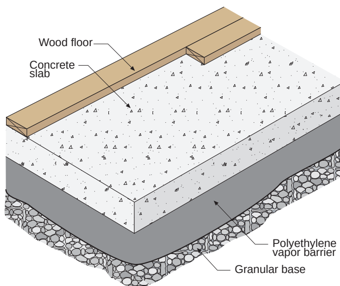
Figure 11.20: Separate the Concrete from the Ground: This needs to be done from underneath and from the sides. We also need dry concrete. We need low water-to-cement ratio concrete or we need to wait for the concrete to dry before we install flooring.
