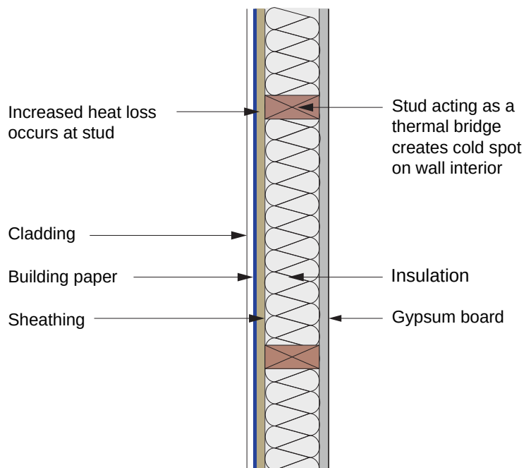
Figure 2.20: Thermal Bridge Through Framing Members - A more common example of thermal bridging is the wood stud of a typical exterior frame wall.
