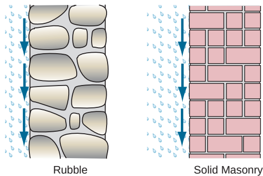
Figure 3.9: Mass/Storage - Rainwater entry controlled by providing materials that can store, absorb, redistribute and dry.
