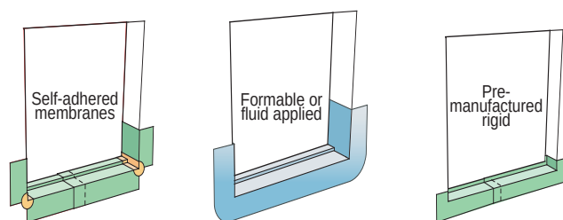
Figure 3.23: Pan Flashing Approaches – Note the back dams and end dams.
