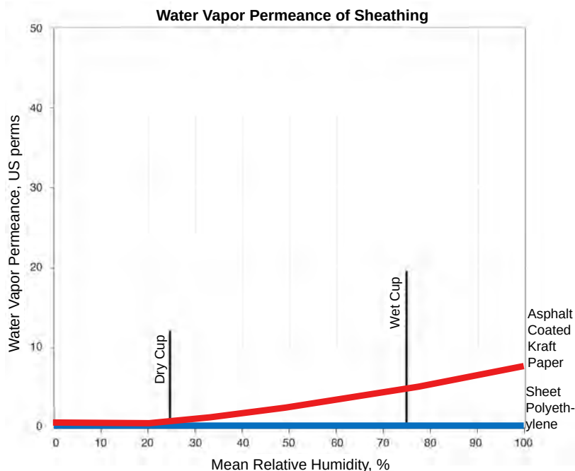
Figure 3.67: Kraft Paper Vapor Transfer - Asphalt coated kraft paper installed on the interior fiberglass batt cavity insulation changes its water vapor permeance as a function of relative humidity.
