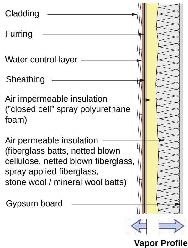
Figure 4.7: Wood Frame Assembly With Interior Spray Foam Cavity Insulation and Siding
