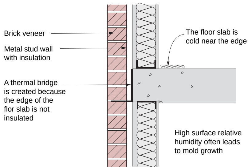
Figure 2.19: Thermal Bridge at Wall/Floor Intersection - Localized cooling of surfaces occurs as a result of thermal bridges. Thermal bridges are regions of relatively high heat flow conductance in a building enclosure. An example of a significant thermal bridge is the edge of a concrete floor slab in residential apartment construction.
