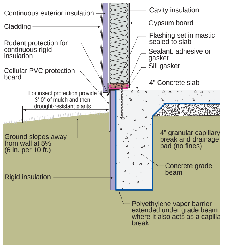
Figure 6.18: Externally Insulated Monolithic Slab Foundation - XPS Rigid Insulation
