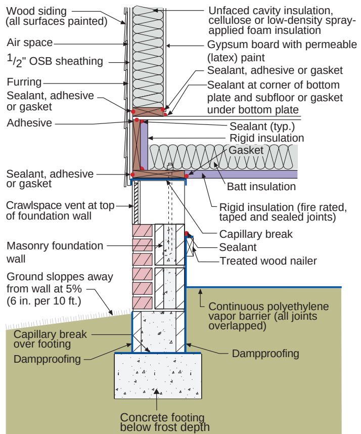
Figure 6.9: Vented Crawlspace – Rigid Insulation
