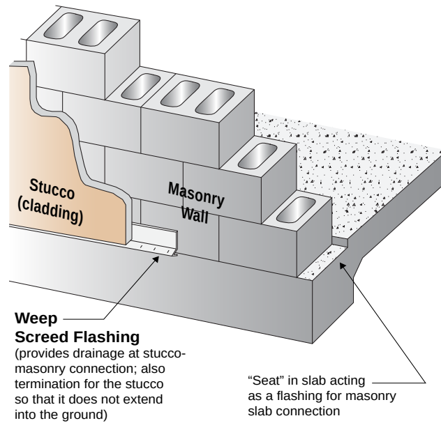
Figure 3.17: Mass/Storage Assemblies – Mass/storage assemblies store, absorb, redistribute and dry rainwater and groundwater without being damaged such as a masonry wall rendered with a Portland cement based stucco.
