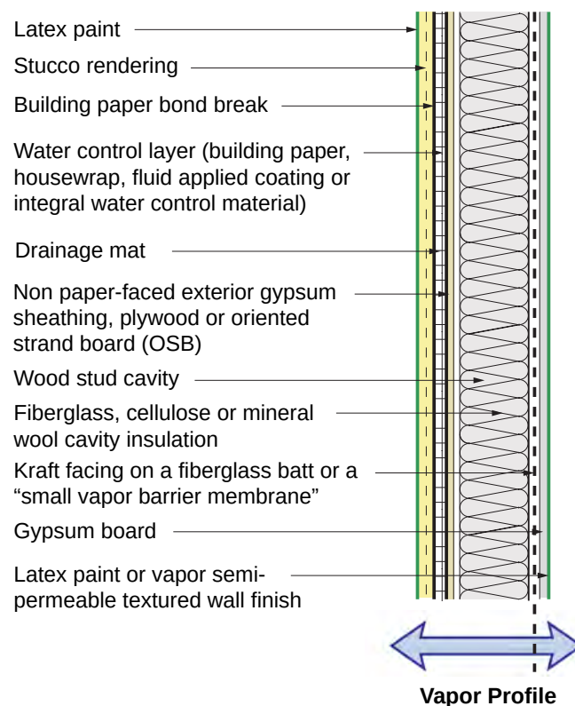
Figure 4.9: Wood Frame Assembly With Interior Cavity Insulation and Stucco With an Interior Vapor Control Layer
