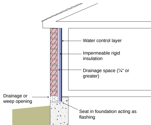
Figure 3.18: Ventilated Cavity – Brick veneer back ventilated to flush inward moving moisture out of the assembly.
