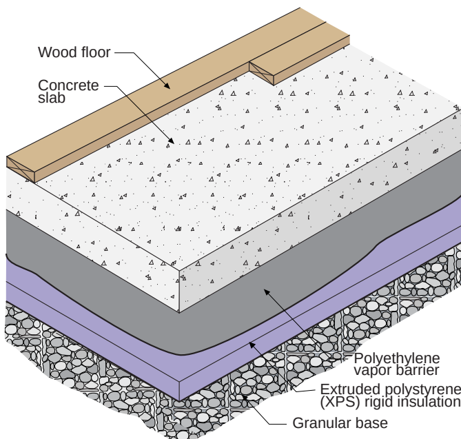
Figure 11.22: Insulating the Slab: Install the insulation under the plastic vapor barrier and over the top of a granular capillary break. Do not install the insulation over the top of the plastic vapor barrier and under the slab. The insulation will get wet. Installing insulation under the vapor barrier allows it to dry into the granular layer.
