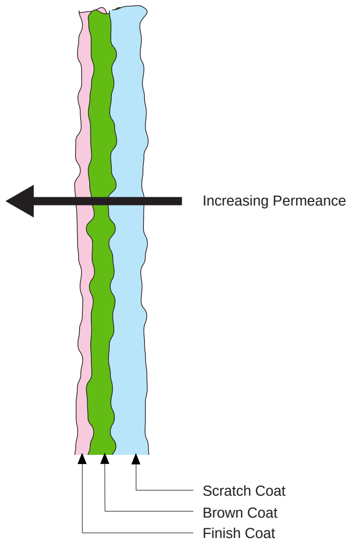
Figure 11.24: Traditional Stucco - Each successive layer to the exterior was more vapor open than the layer it covered.
