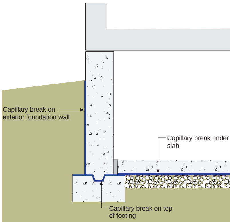
Figure 3.34: Capillary Breaks Below Grade - Capillary suction in concrete foundation walls is traditionally controlled by dampproofing the exterior surface of the wall where it is in contact with the surrounding damp soil.
