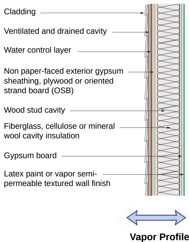
Figure 4.2: Wood Frame Assembly With Interior Cavity Insulation and Siding
