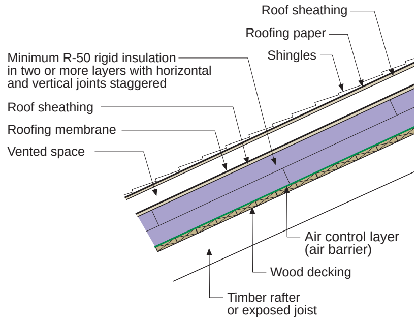
Figure 5.3: Unvented Roof – Vented over-roof constructed over unvented under-roof.
