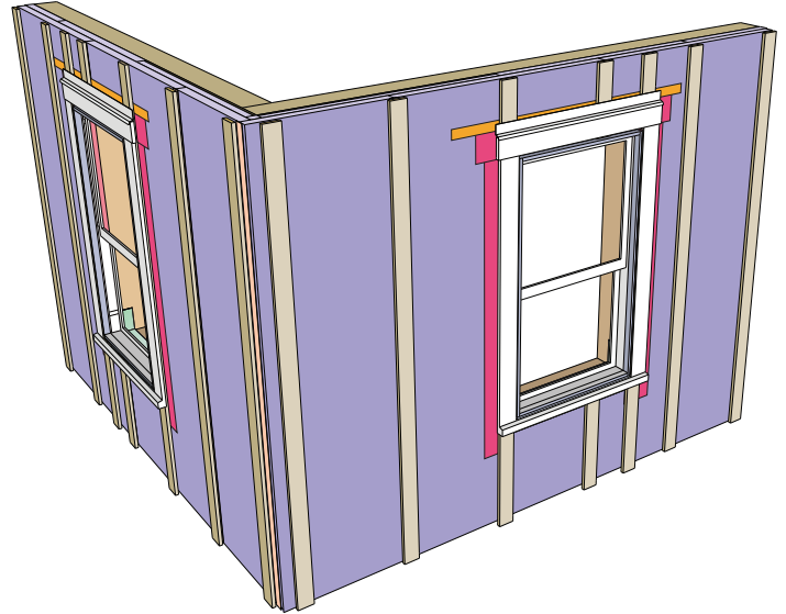
Figure 11.31c: Window Trim Installed – Note that the flashing above the horizontal trim at the top of the window is installed to protect the trim - not to protect the window unit.
