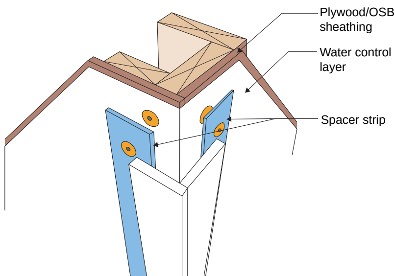
Figure 3.38: Wood Trim Over Air Space – Air space serves as a receptor for capillary moisture.
