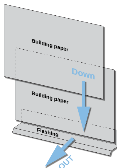
Figure 3.12: Flashing Integration - Flashings need to be integrated with water control layers such as building papers.
