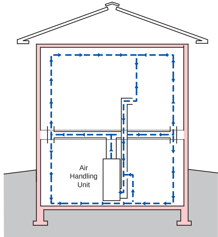
Figure 3.51: Mechanical System Pressure Effects – Interior air circulation system.
