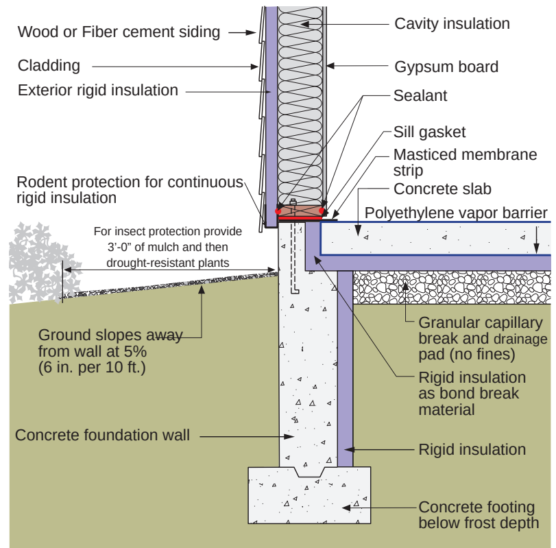
Figure 9.2: Stem Wall Foundation – Internally insulated.
