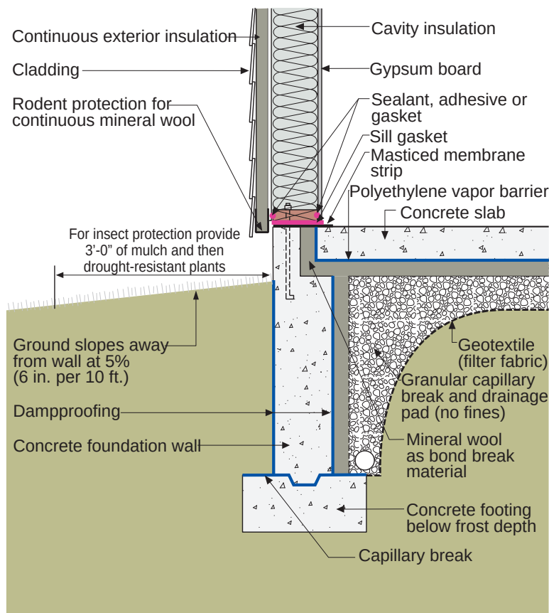
Figure 6.17: Insulated Stem Wall Slab Foundation – Mineral Wool Rigid Insulation
