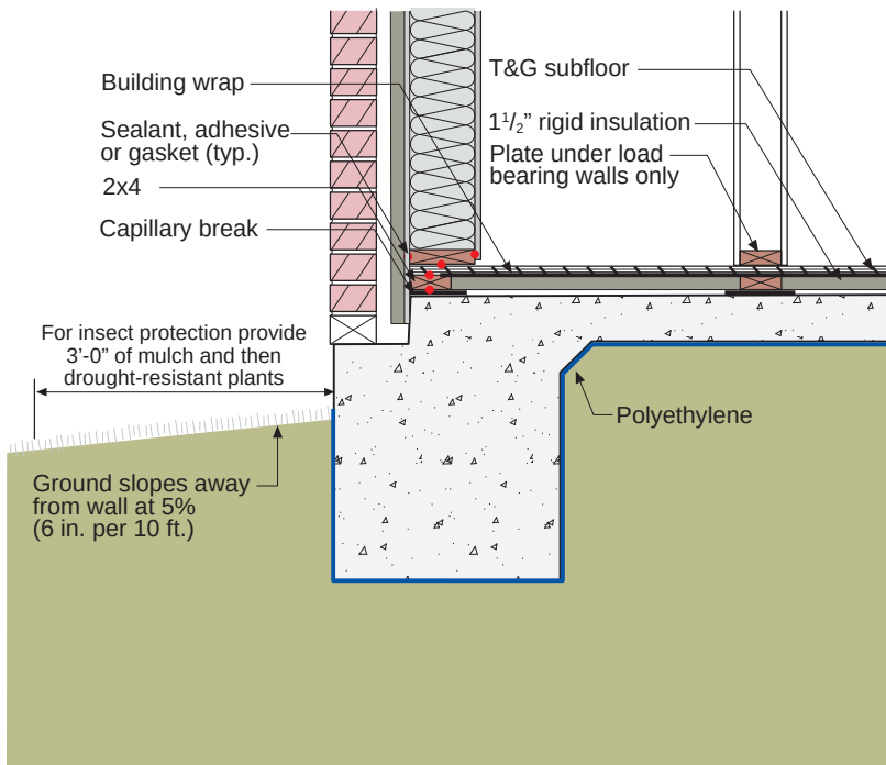
Figure 6.23: Topside Insulated Monolithic Slab Foundation with Brick Veneer – Mineral Wool Rigid Insulation
