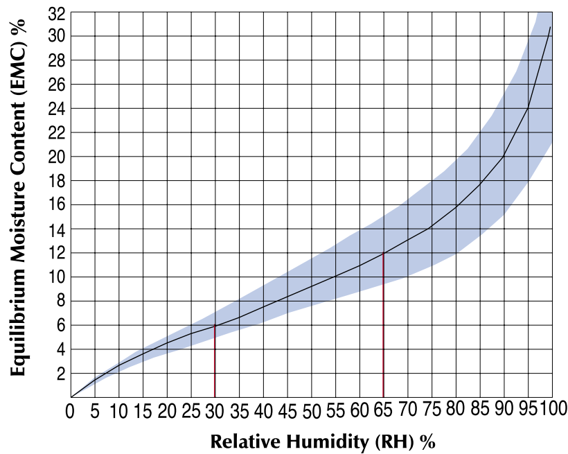
Figure 11.23: Conditioning the Wood Flooring: Wood expands and contracts with relative humidity changes as it is a hygroscopic material. In most places the interior winter relative humidity is low (typically 30 percent) and high during the summer (typically 65 percent). The wood flooring is going to float between 6 percent moisture content by weight and 12 percent moisture content by weight - a 6 percent seasonal swing. If wood flooring is installed at 6 percent it will buckle when it goes to 12 percent. If wood flooring is installed at 12 percent it will shrink and leave big gaps when it goes to 6 percent. Condition wood to the mid-range moisture content it is likely to see during service. For most of the lower 48 states that is 9 percent moisture content by weight.
