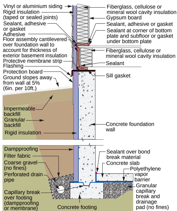
Figure 10.6: Basement Foundation – Externally insulated.
