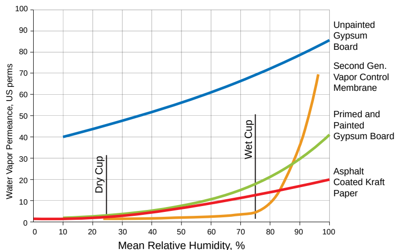
Figure 2.10: Permeance of Interior Wall Linings - The kraft facing has a “dry cup” value of 1 perm and a “wet cup” value of 15 perms. In most of the United States and Canada buildings in the winter have low interior relative humidities – around 25 percent and high interior relative humidities during the summer – 60 percent and higher. The kraft facing works much like a “valve”....closed in the winter and open in the summer.
