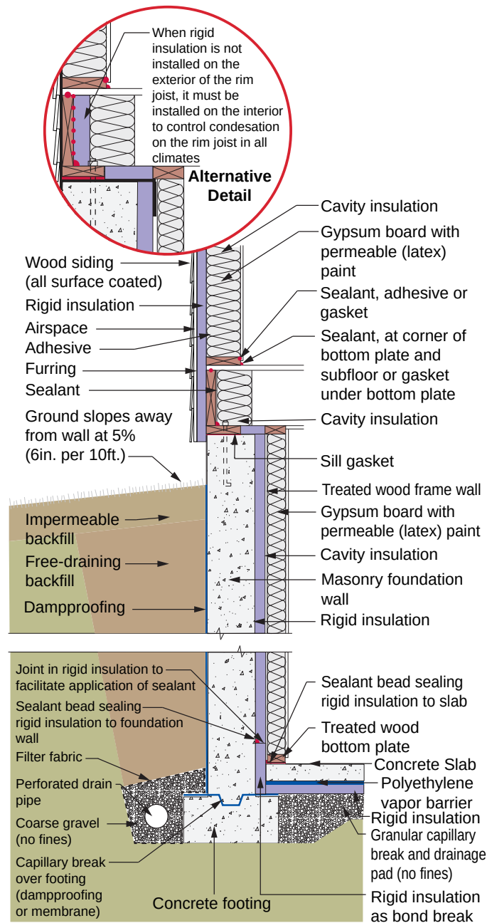
Figure 9.5: Basement Foundation – Internally insulated.
