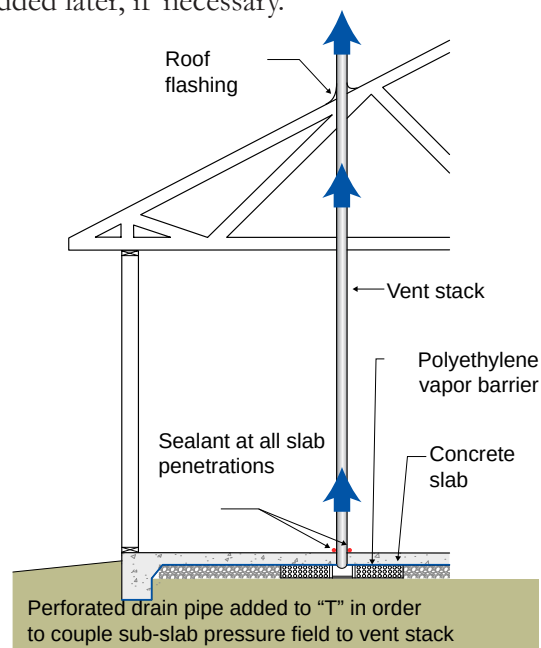
Figure 6.1: Soil Gas Control – Approach for slab foundations.
