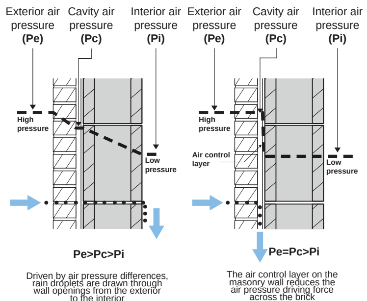
Figure 3.7: Air Pressure – A driving force for rain entry.
