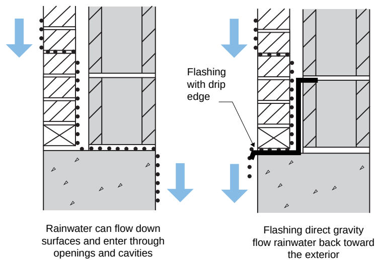
Figure 3.6: Gravity – A driving force for rain entry.
