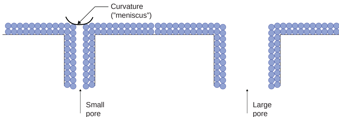
Figure 2.6: Capillary Condensation – Small pores get filled before large pores. A reduction in vapor pressure over a curved surface results in capillary condensation. Thank Lord Kelvin for this. Once again the real world is not as “crisp” and “clean” as drawn.
