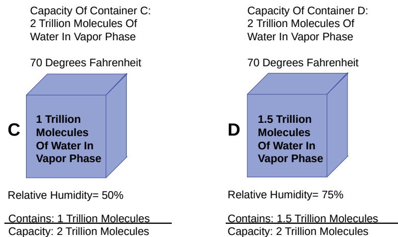
Figure 2.14: Relative Humidity Increases as Vapor Pressure or Moisture Content of Air Increases - The concept of relative humidity, vapor pressure, and the influence of temperature and vapor pressure on relative humidity.
