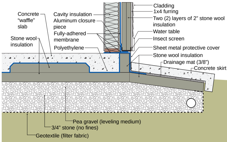
Figure 6.25: Shallow Frost Protected Slab Foundation – Mineral Wool Rigid Insulation
