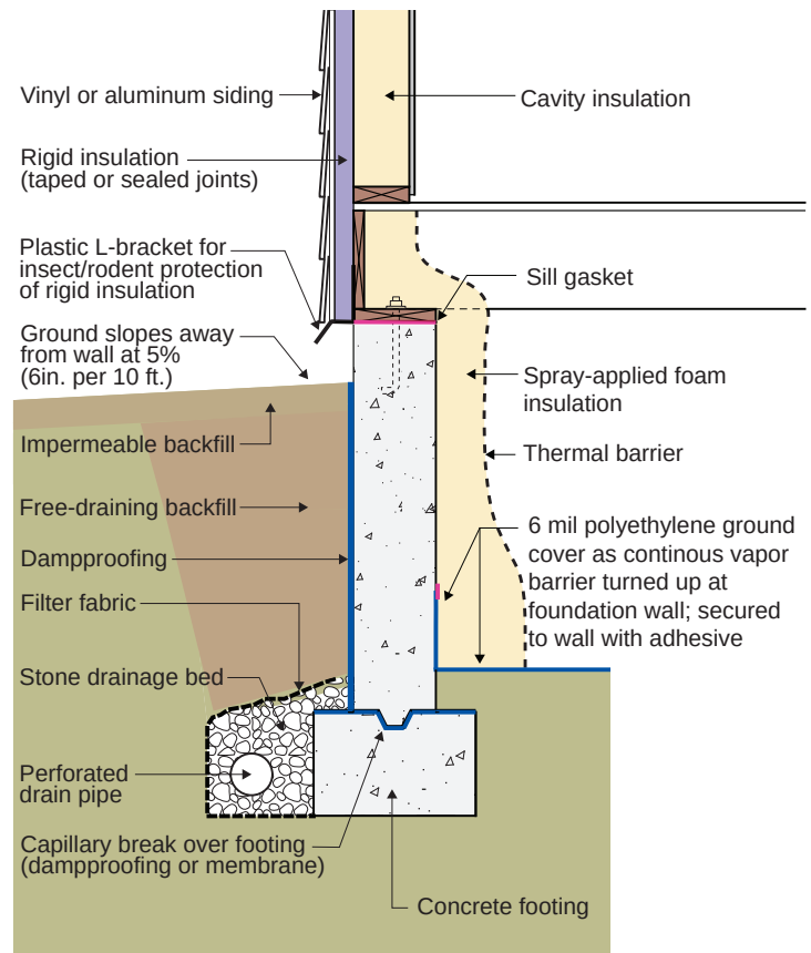
Figure 6.13: Conditioned Crawlspace – Spray Polyurethane Foam
