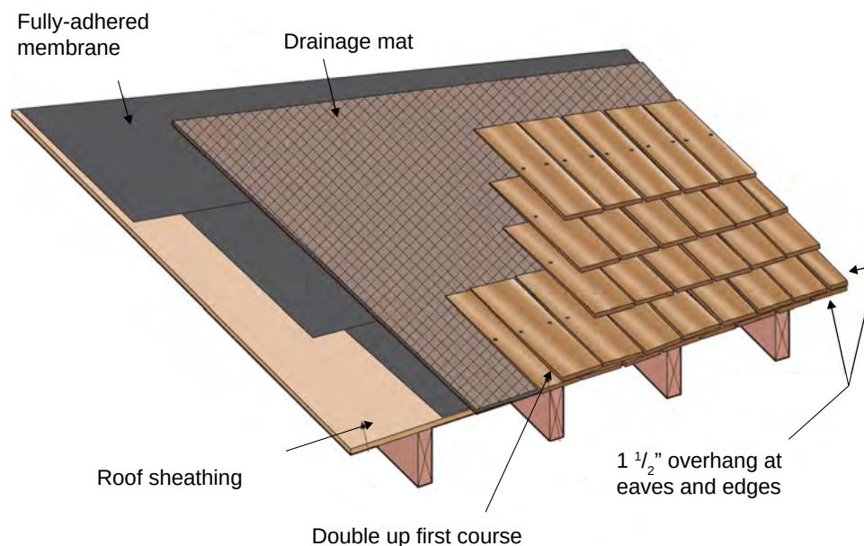
Figure 3.40: Sheet Goods and Wood Shingles and Shakes - Where sheet goods are used for roof sheathing such as plywood or oriented strand board (OSB) in conjunction with wood shakes and shingles an air gap must be added between the shakes and shingles to act as a receptor for the capillary moisture. The air gap is typically provided using a breathable drainage mesh.
