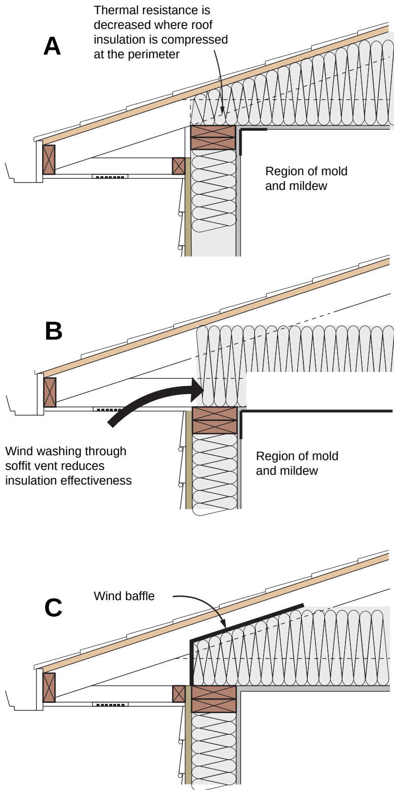
Figure 2.18: Heat Loss Effects Where Walls Intersect Roofs - Cool interior surfaces in heating climates also can occur where exterior walls intersect roofs.
