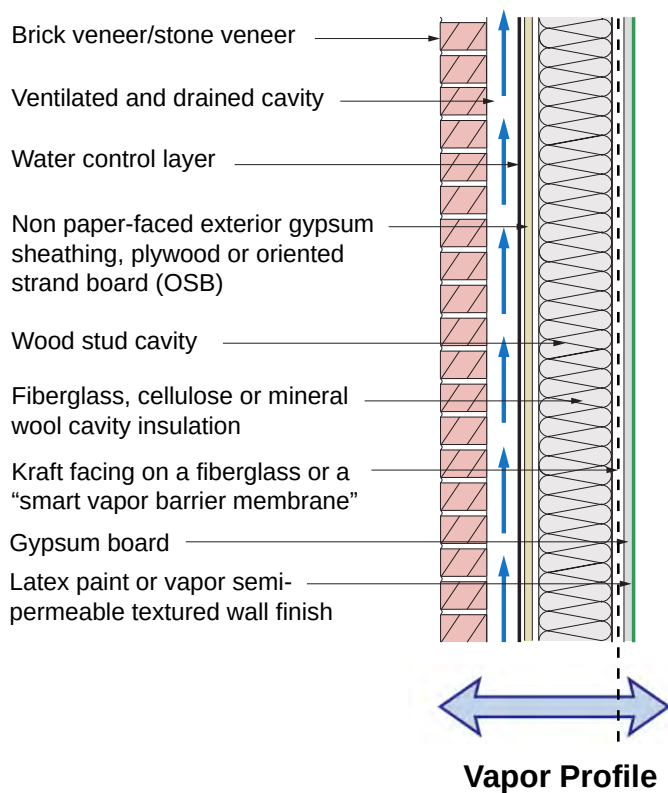
Figure 4.4: Wood Frame Assembly With Interior Cavity Insulation and Brick or Stone Veneer With an Interior Vapor Control Layer
