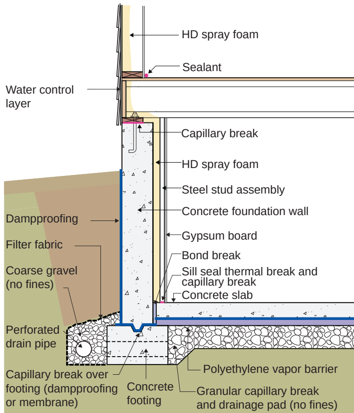
Figure 6.5: Concrete Basement With Interior Spray Polyurethane Foam Insulation
