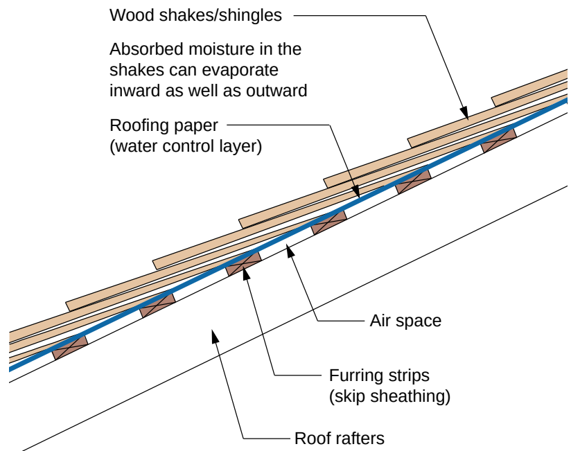
Figure 3.39: Wood Shingles and Shakes - The wood shakes and shingles absorb deposited rainwater due to capillary suction. The wood shakes and shingles dry to both directions.
