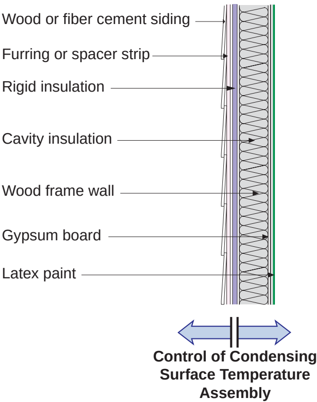
Figure 9.9: Wood Frame Wall – Control of condensing surface temperature assembly.
