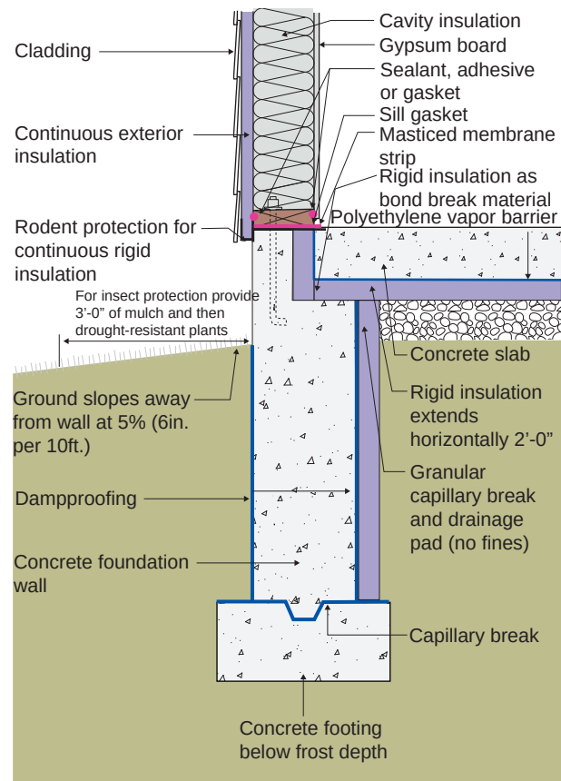
Figure 6.16: Insulated Stem Wall Slab Foundation – XPS and EPS Rigid Insulation
