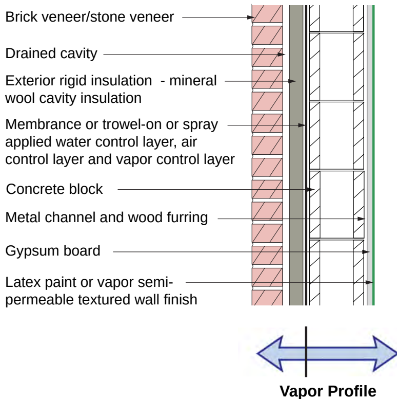
Figure 4.19: Concrete Masonry Unit (CMU) With Exterior Insulation and Brick or Stone Veneer
