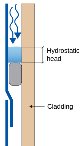
Figure 3.2: Hydrostatic Pressure Behind Cladding - If rainwater penetrates a cladding system and drainage is not provided water can build up creating hydrostatic pressure.
