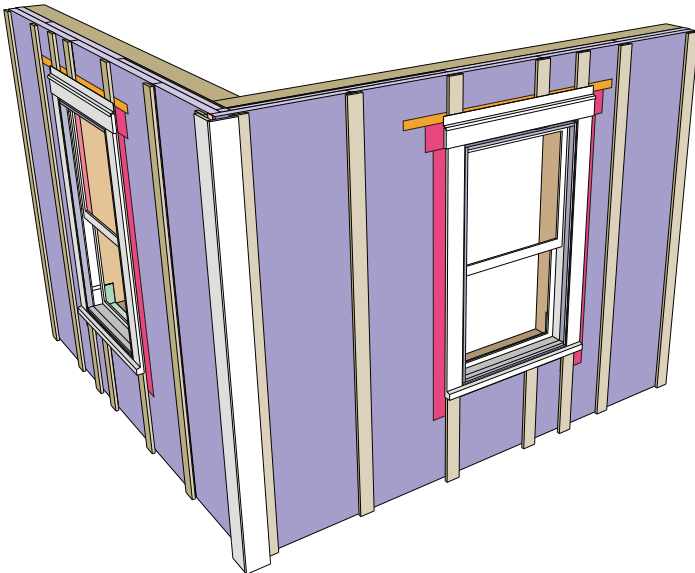
Figure 11.31d: Corner Trim Installed – The two corner trim pieces are attached “to themselves” and then the “L-shaped” trim assembly is attached to the gapped wood furring at the corner.
