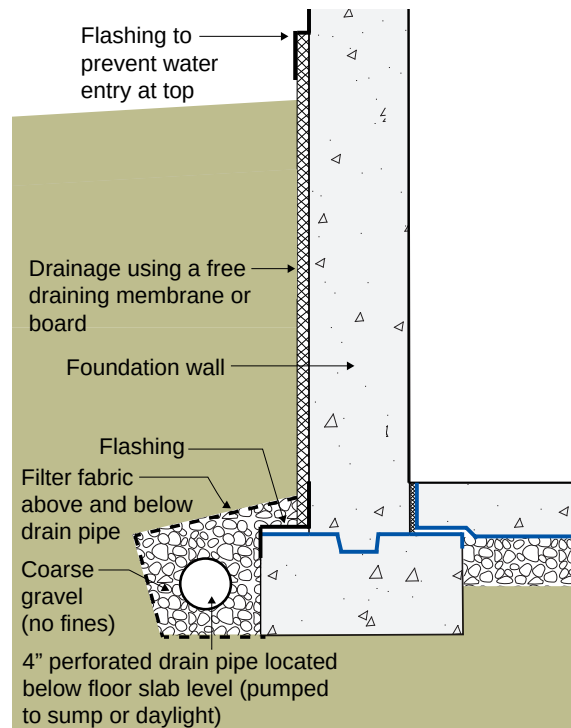
Figure 3.29: Free Draining Materials – Note the cap flashing and connection to perimeter drainage systems.
