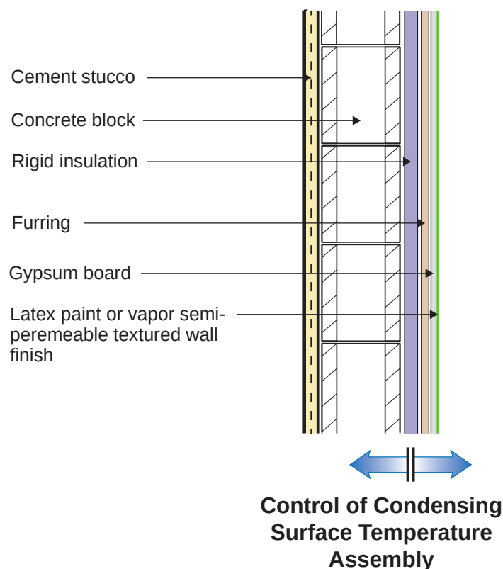
Figure 8.10: CMU Wall – Internally insulated.
