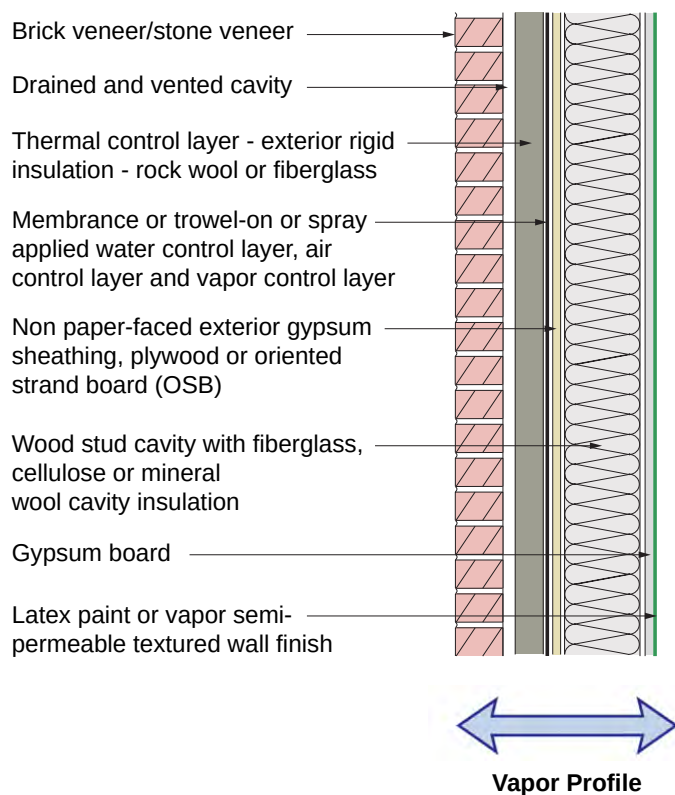
Figure 4.14: Wood Frame Assembly With Exterior Insulation and Interior Cavity Insulation With Brick or Stone Veneer and No Interior Vapor Control Layer
