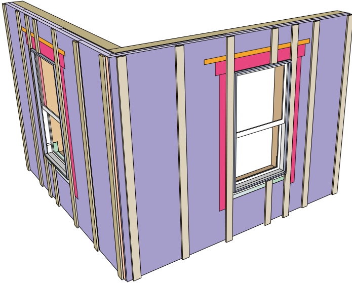
Figure 11.31b: Furring Strip Spacers – Note the corner geometry of the wood furring. The furring is gaped laterally at the corner.
