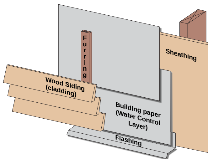
Figure 3.16: Screen Assemblies - Screen assemblies have multiple layers dedicated to water management.
