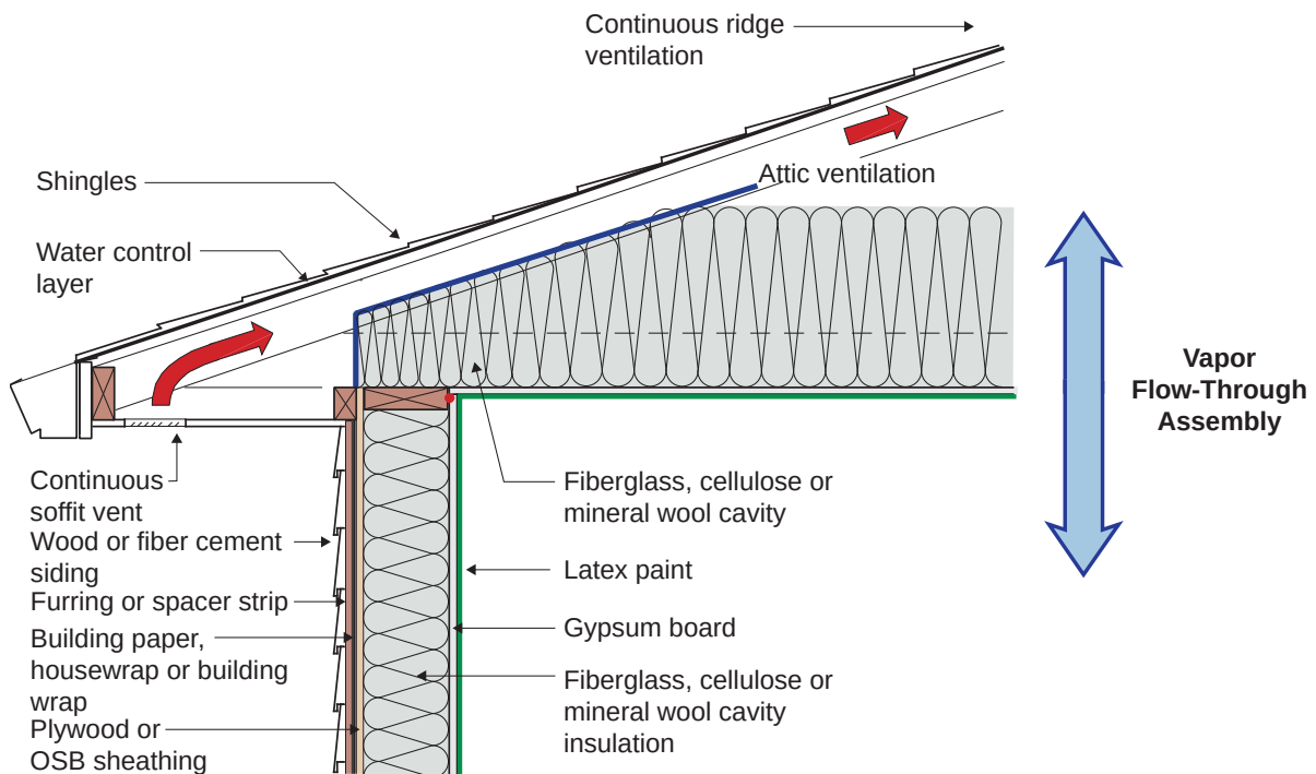
Figure 3.62: Flow-Through Assembly - An attic assembly that is vented and constructed with latex painted ceiling gypsum board and insulated with fiberglass batts or cellulose is also called a flow-through assembly.
