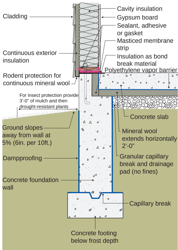
Figure 6.15: Insulated Stem Wall Slab Foundation – Mineral Wool Rigid Insulation
