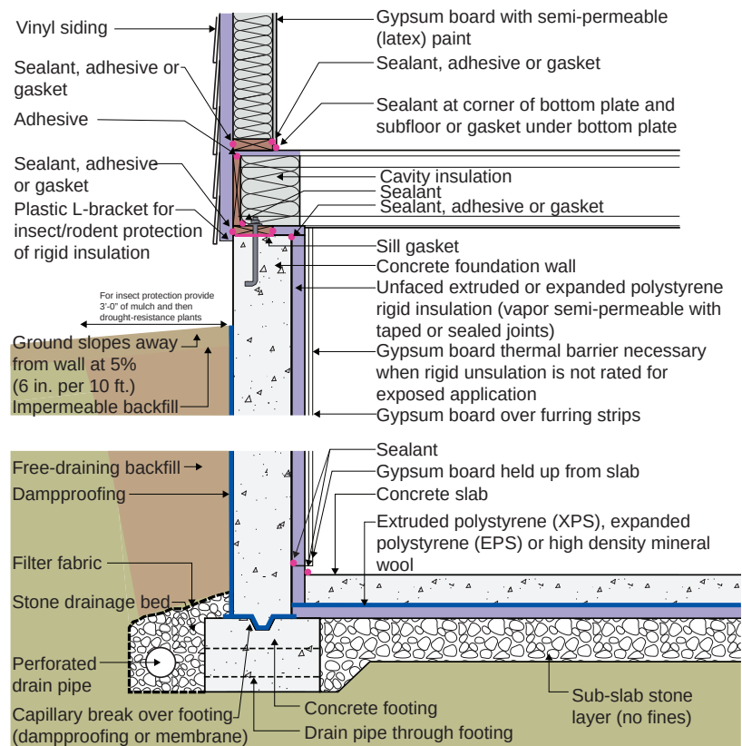
Figure 6.4: Concrete Basement With Interior Rigid Insulation
