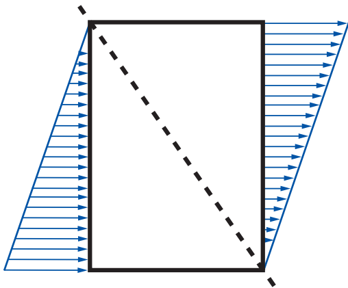
Figure 3.50: Wind And Stack Effect - The when wind effects are combined with the stack effect the wind tends to “tilt” the neutral pressure plane.
