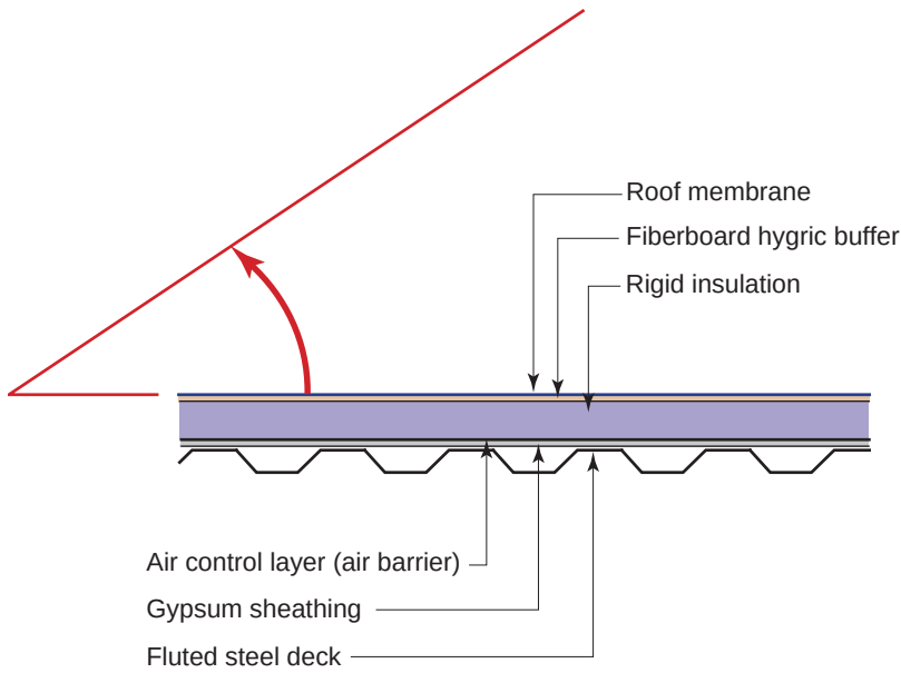
Figure 5.1: Unvented Roof – Standard commercial compact roof design
