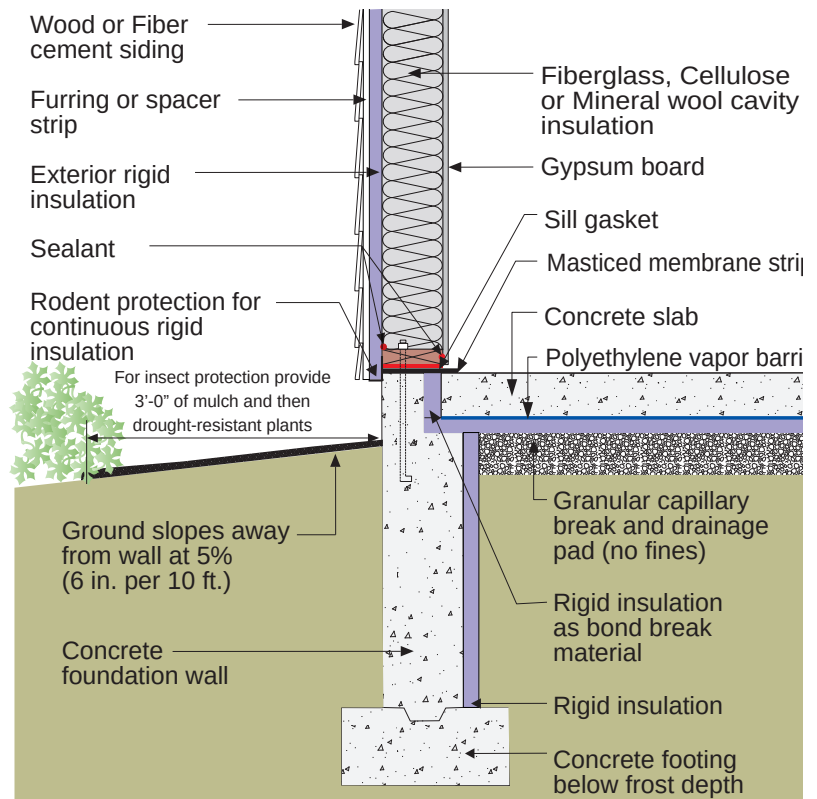
Figure 10.2: Stem Wall Foundation – Internally insulated.
