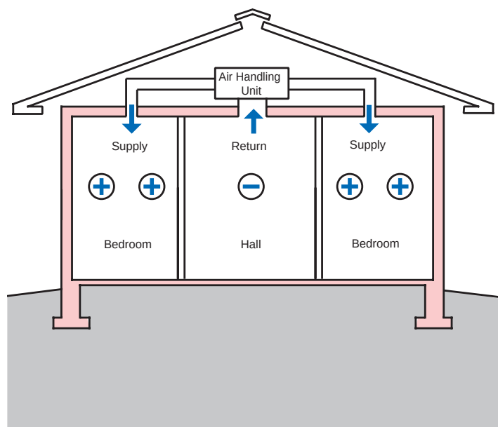
Figure 3.54: Pressurization of Bedrooms – Unbalanced airflows due to supply registers by no return registers.
