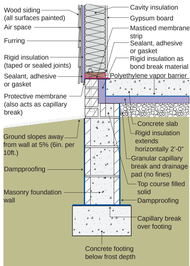
Figure 6.14: Insulated Stem Wall Slab Foundation – XPS and EPS Rigid Insulation
