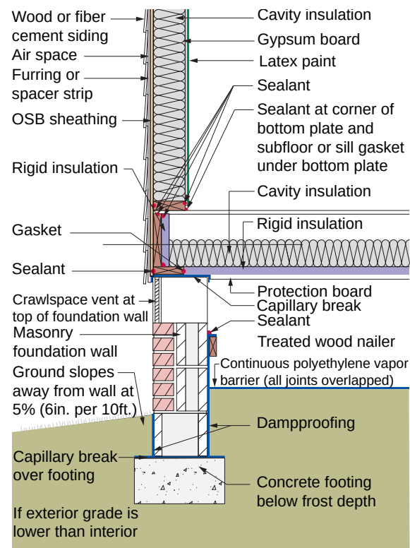
Figure 9.3: Crawl Space Foundation – Vented crawl space.
