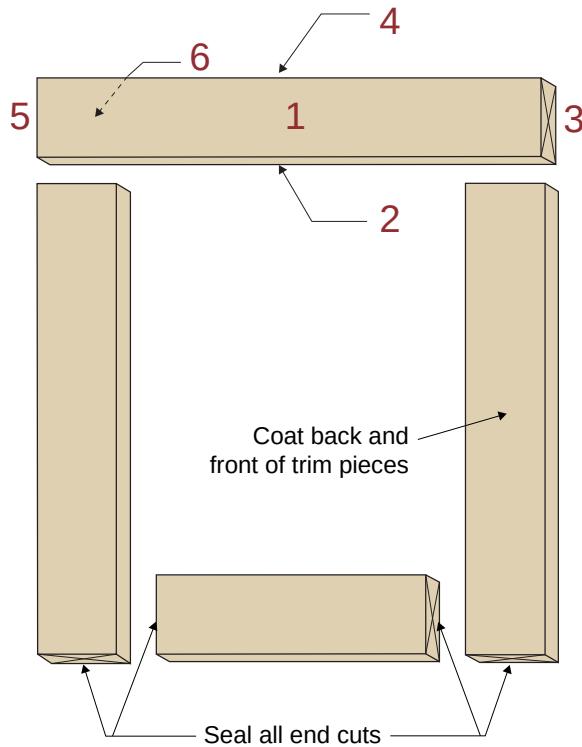
Figure 3.37: Wood Trim - All six surfaces of the trim (the front, the back, the edges and the end cuts) should be sealed
