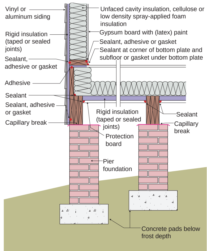
Figure 6.11: Vented Crawlspace – Pier Foundation - Rigid Insulation
