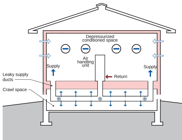
Figure 3.56: Depressurization of Crawlspace Buildings – Leaky ductwork located in vented crawlspaces leads to depressurization.
