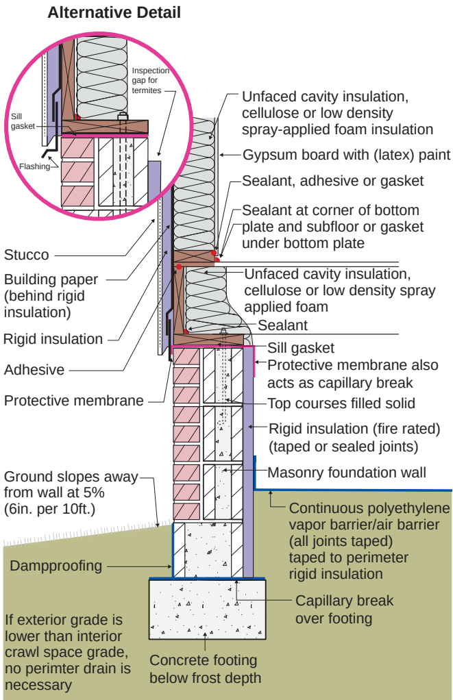
Figure 6.12: Conditioned Crawl space – Rigid Insulation
