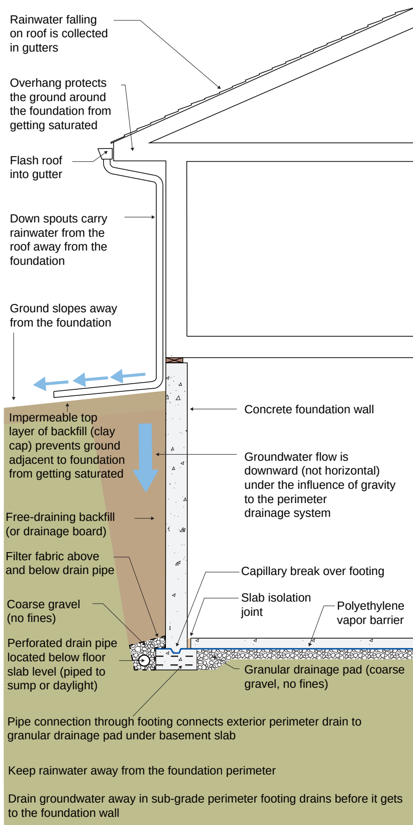
Figure 3.28: Basements – Water management for basement construction.
