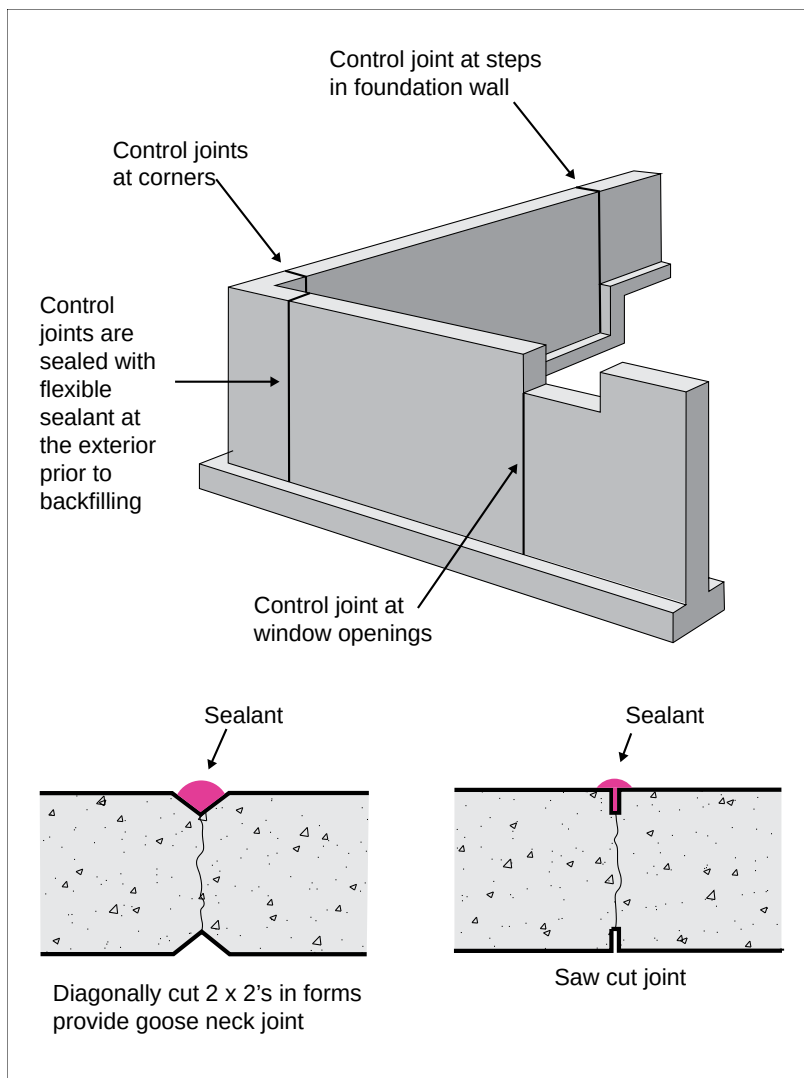
Figure 3.31: Foundation Control Joints - These cracks are repaired or sealed prior to backfilling.
