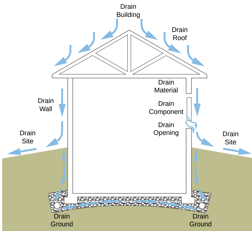
Figure 3.10: Drainage - Everything should be drained: the site, the ground, the building, the assemblies, the openings, the components and the materials.
