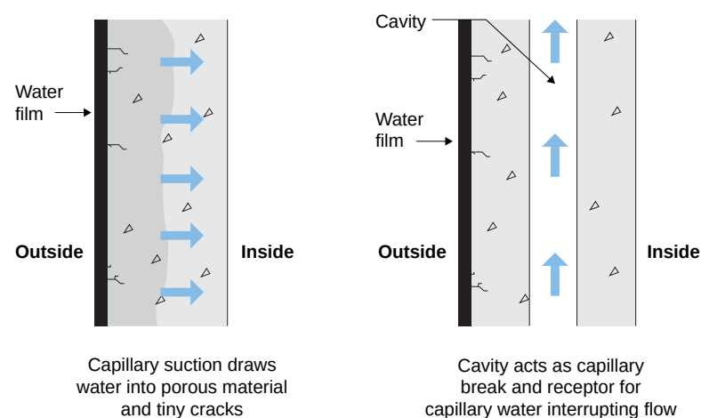
Figure 3.5: Capillarity – A driving force for rain entry.
