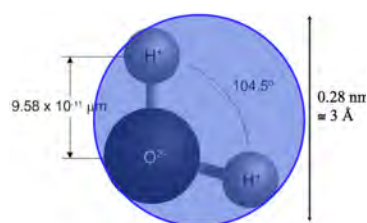
Figure 2.1: The Water Molecule – A permanent dipole.
