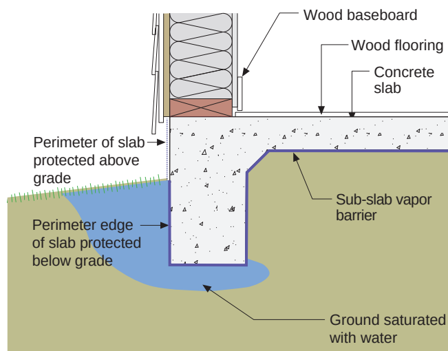
Figure 11.17: Monolithic Slab: A continuous polyethylene vapor barrier and capillary break needs to wrap the entire concrete surface that contacts the ground – especially the perimeter. It is also recommended to paint the exposed edge of the slab above grade to keep it from getting wet from “splash back” (rainwater hitting the ground and bouncing back up) and enthusiastic over irrigation by occupants. The paint should be “liquid water” closed and “vapor water” open – hygrophobic and vapor permeable – typical acrylic latex paint formulated for concrete substrates
