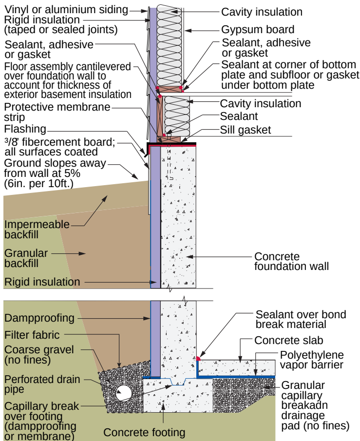
Figure 9.6: Basement Foundation – Externally insulated.
