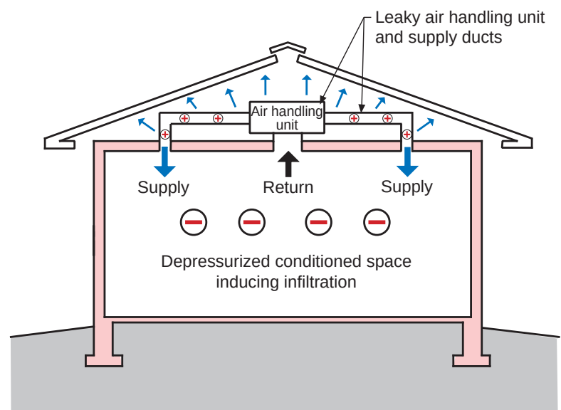
Figure 5.4: Vented Attic – Mechanical system and leaky ductwork located in vented attic space.
