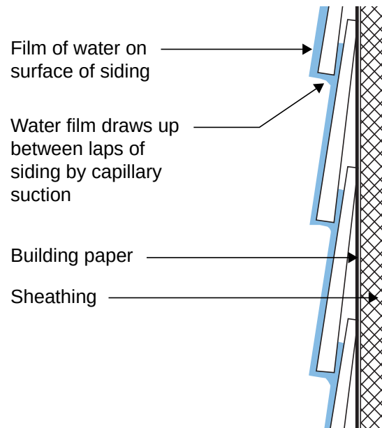
Figure 11.28: Capillary Rise In Siding – Water is pulled upwards between the laps of siding by capillarity.
