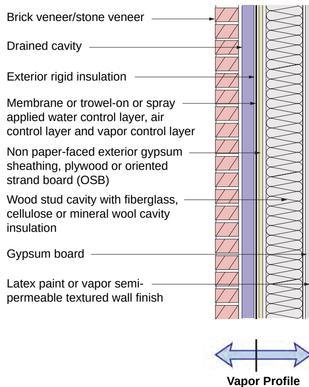
Figure 4.10: Wood Frame Assembly With Exterior Insulation and Interior Cavity Insulation With Brick or Stone Veneer and No Interior Vapor Control Layer
