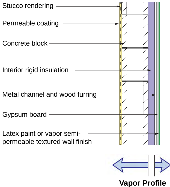
Figure 4.20: Concrete Masonry Unit (CMU) With Interior Rigid Insulation and Stucco
