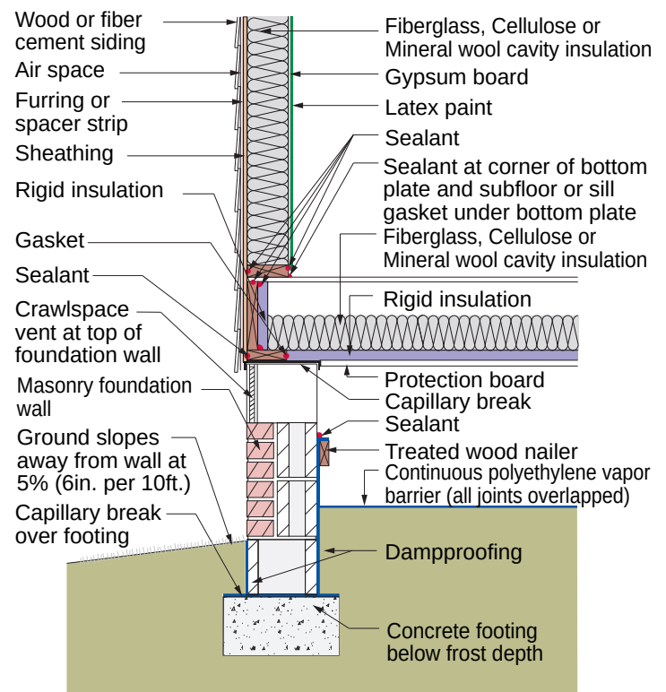
Figure 10.3: Crawl Space Foundation – Vented crawl space.
